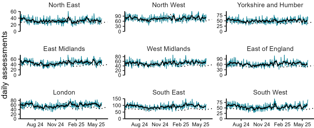
NHS 111 online: diarrhoea by UKHSA region 27/05/2024 to 26/05/2025
