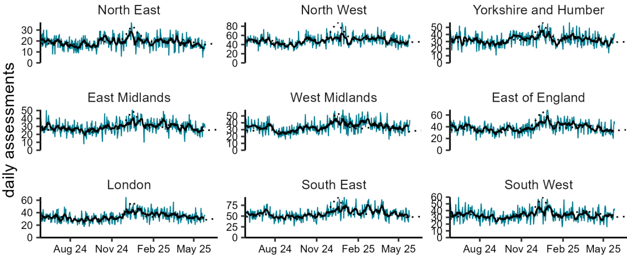
NHS 111 online: vomiting by UKHSA region 27/05/2024 to 26/05/2025
