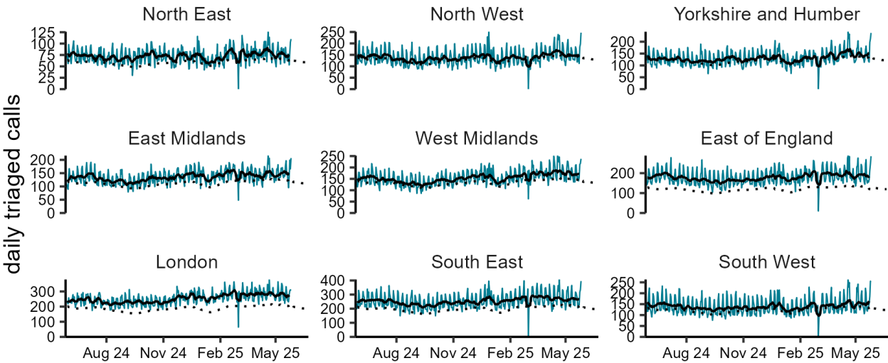
NHS 111 triaged calls: diarrhoea by UKHSA region 27/05/2024 to 26/05/2025
