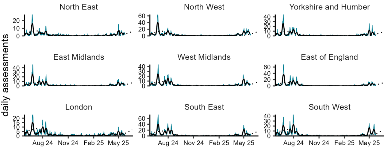
(c) NHS 111 online: heat exposure or sunburn by UKHSA region 27/05/2024 to 26/05/2025
