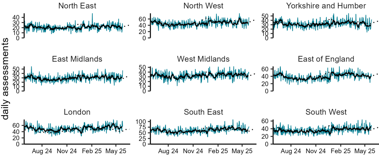
NHS 111 online: eye problems by UKHSA region 27/05/2024 to 26/05/2025
