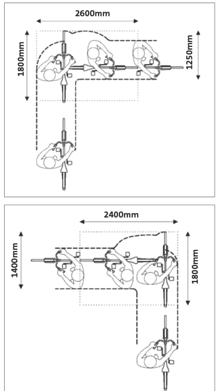
Fig 10: Examples of swept paths of standard sized cycle being pushed (Drawings © Transport Initiatives)
