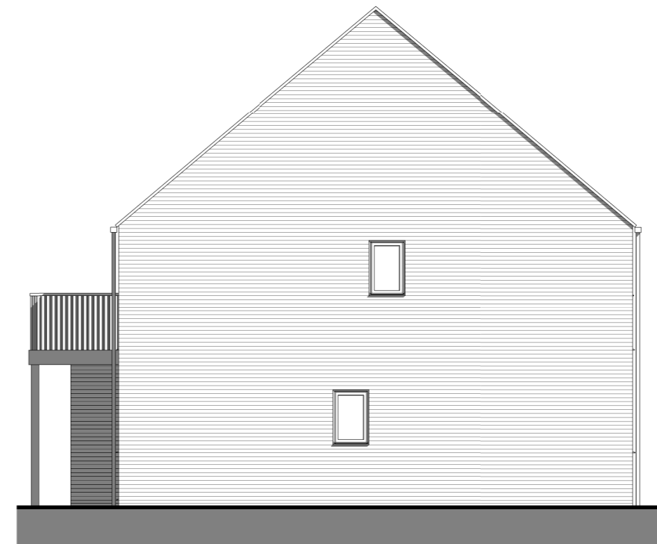
Side Elevation 1 : 100
