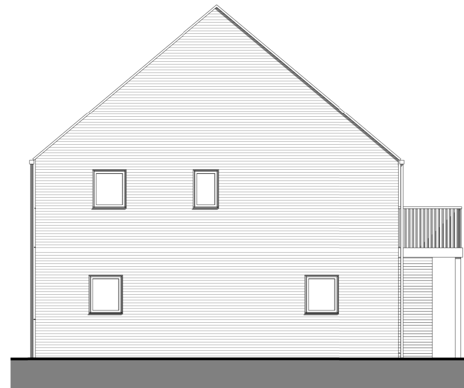
Side Elevation 1 : 100
