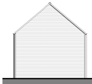
Side Elevation 1 : 100
