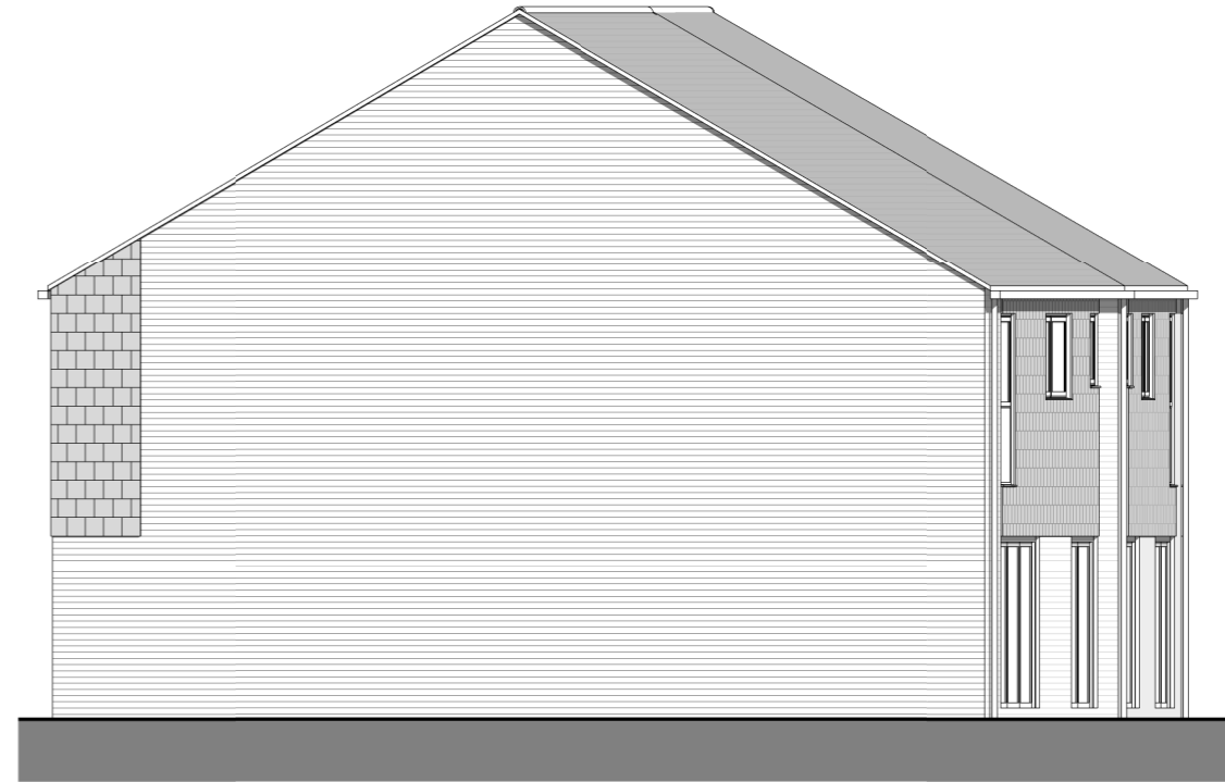
Side Elevation 1 : 100
