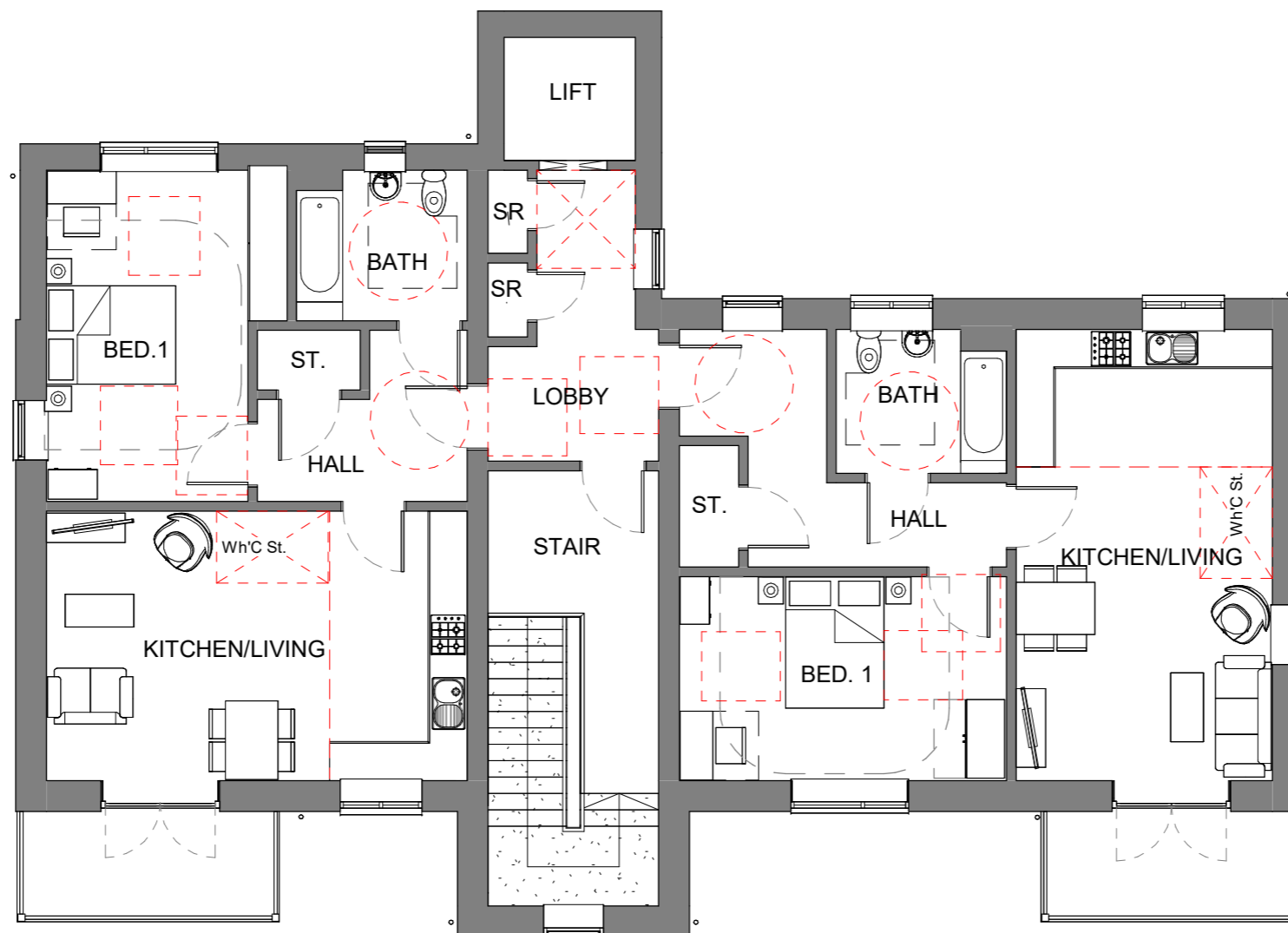
Second Floor 1 : 100
