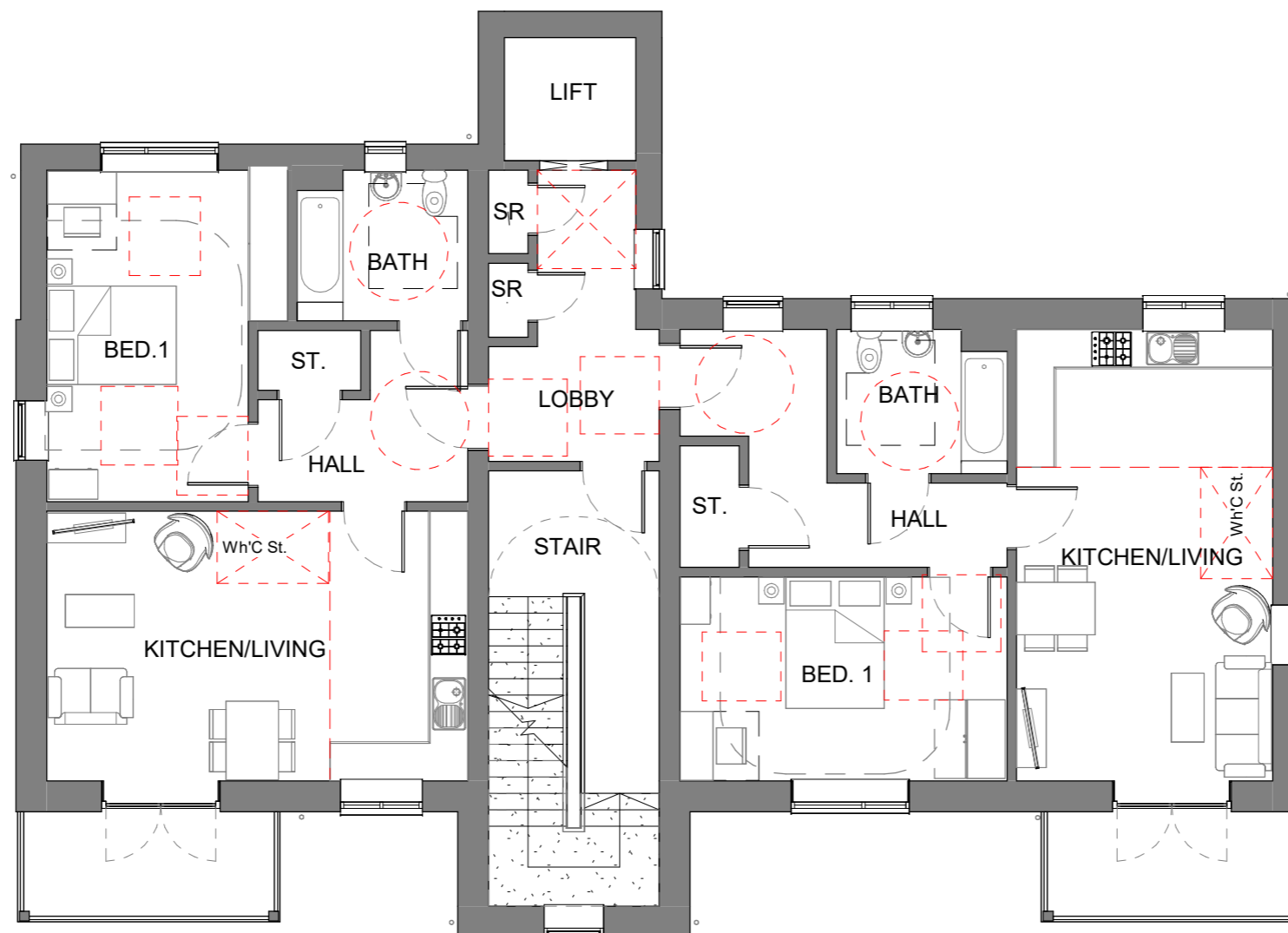
First Floor 1 : 100
