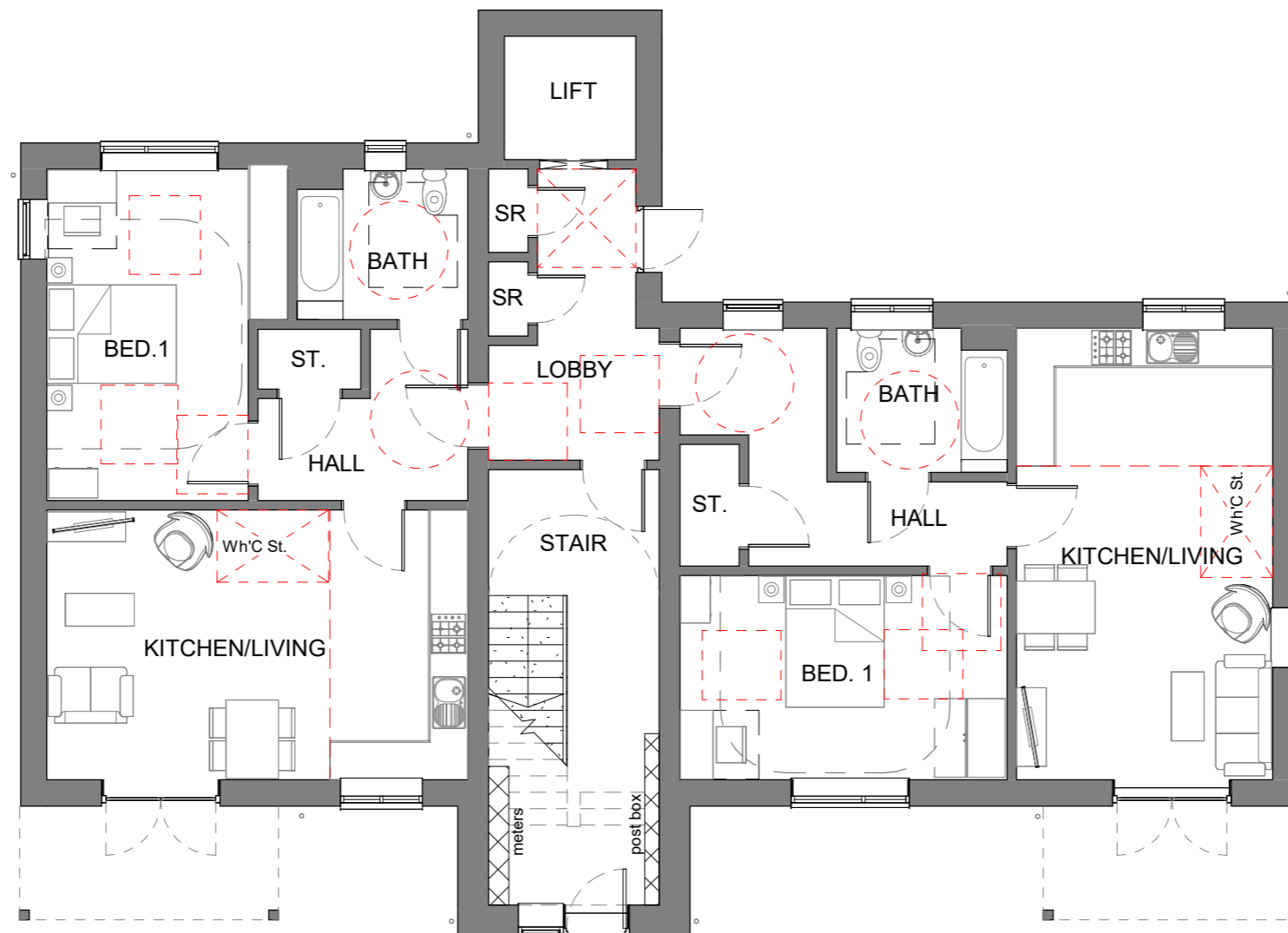
Ground Floor 1 : 100
