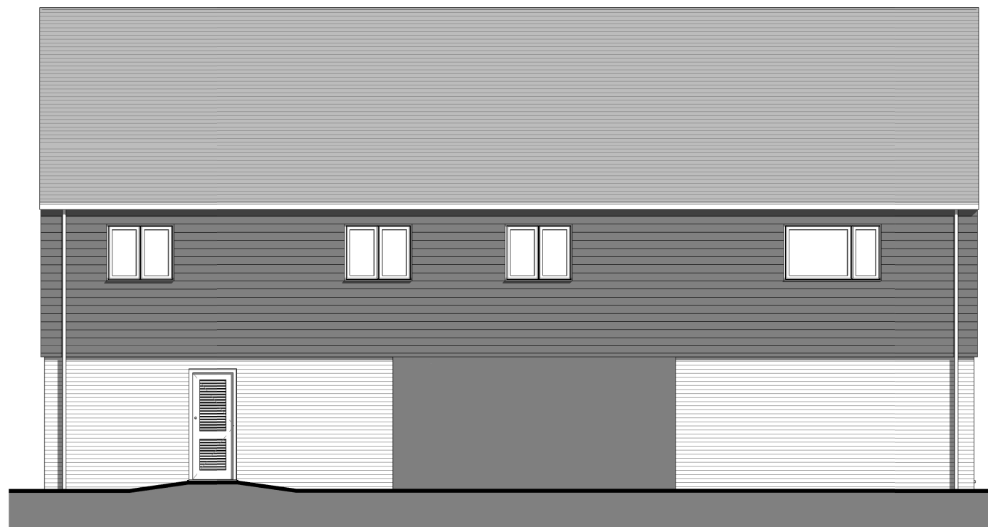
Rear Elevation 1 : 100
