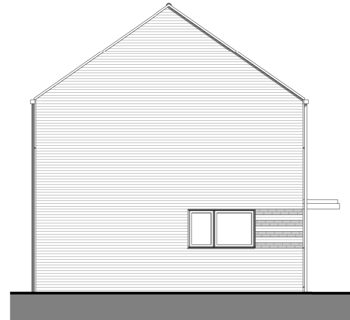
Side Elevation 1 : 100
