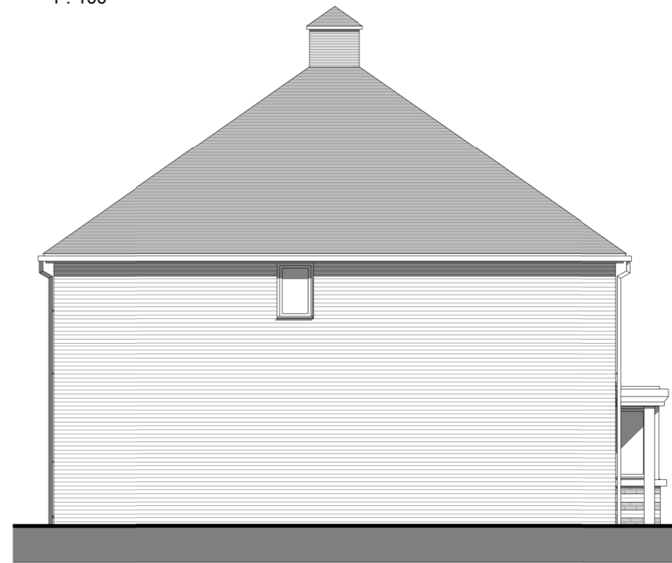
Side Elevation 1 : 100
