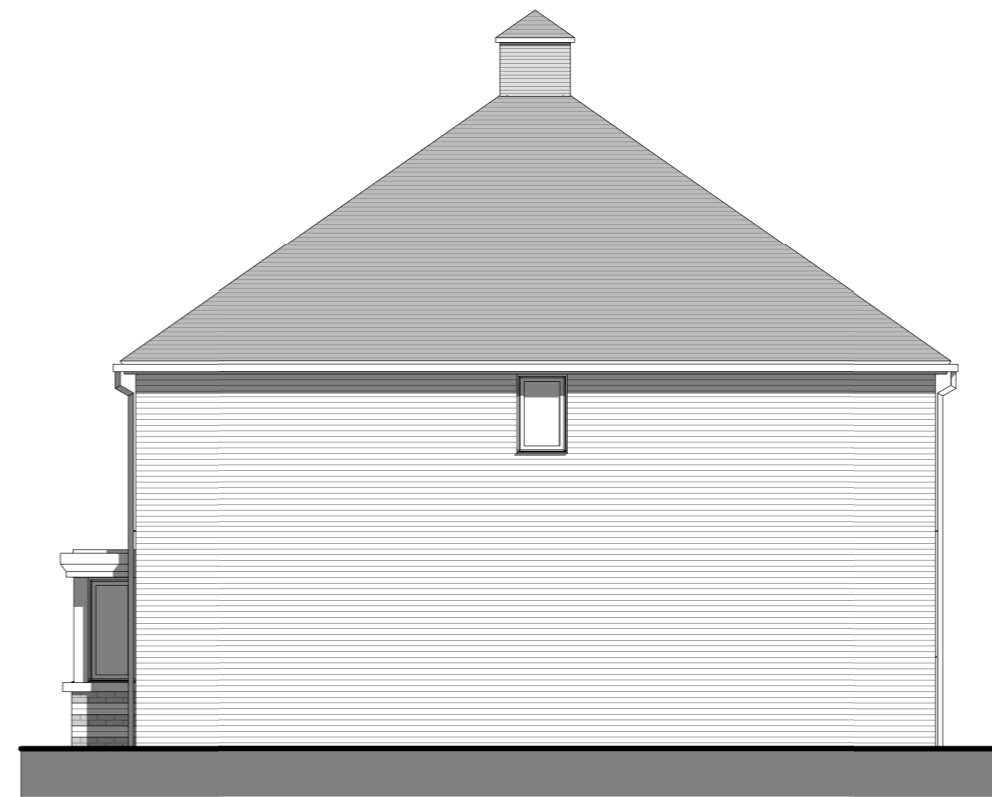
Side Elevation 1 : 100
