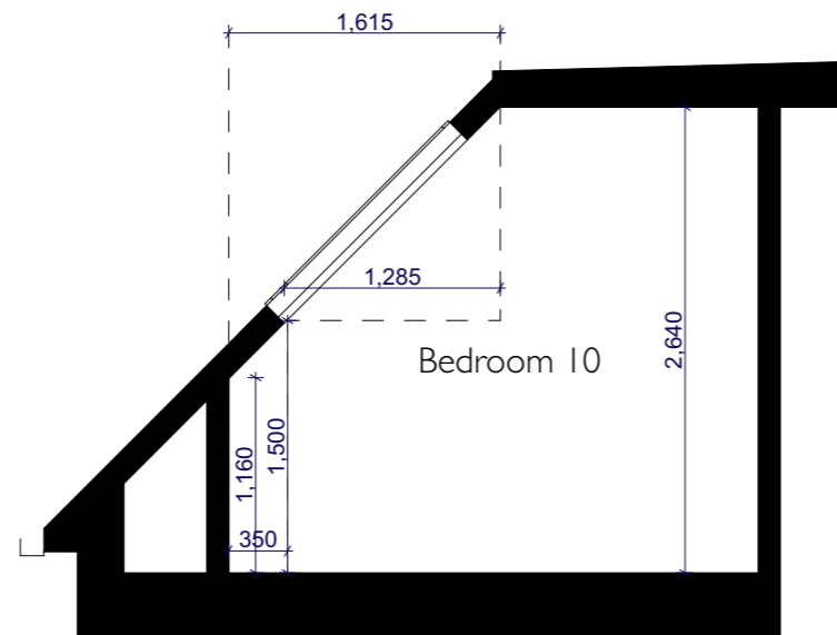
Proposed Second Floor Section S-01
