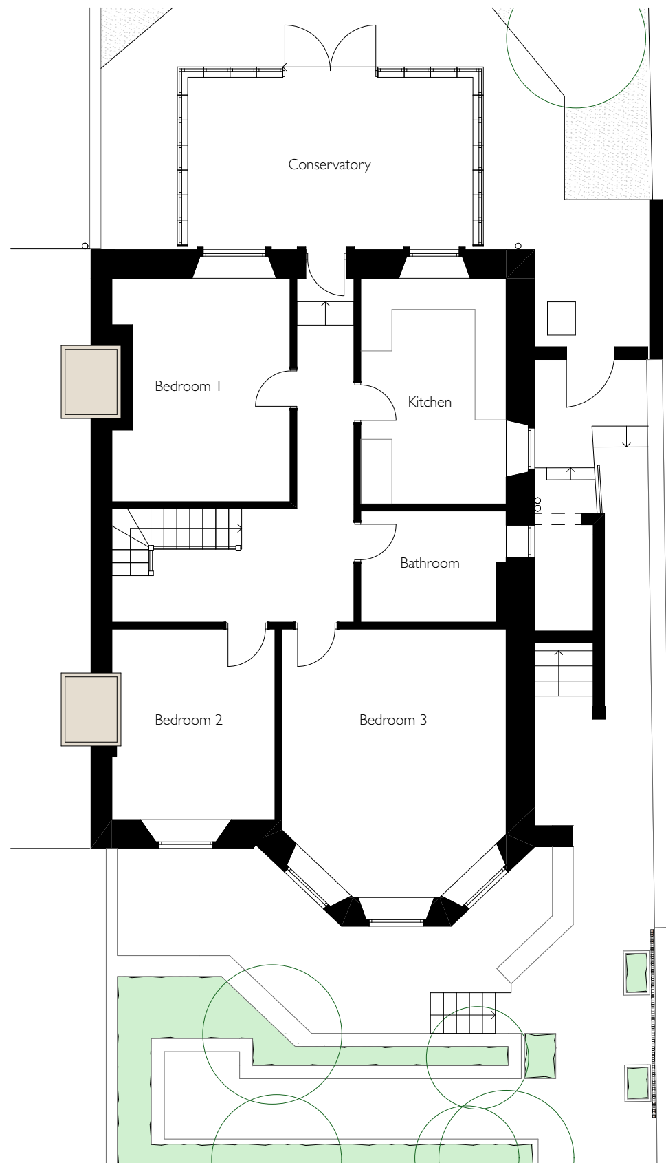
Existing Lower Ground Floor Plan
