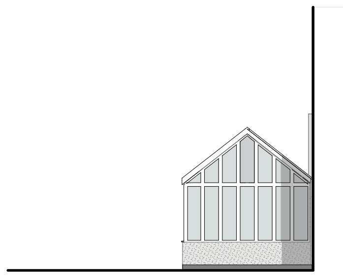
Proposed Side B/North-West Elevation
