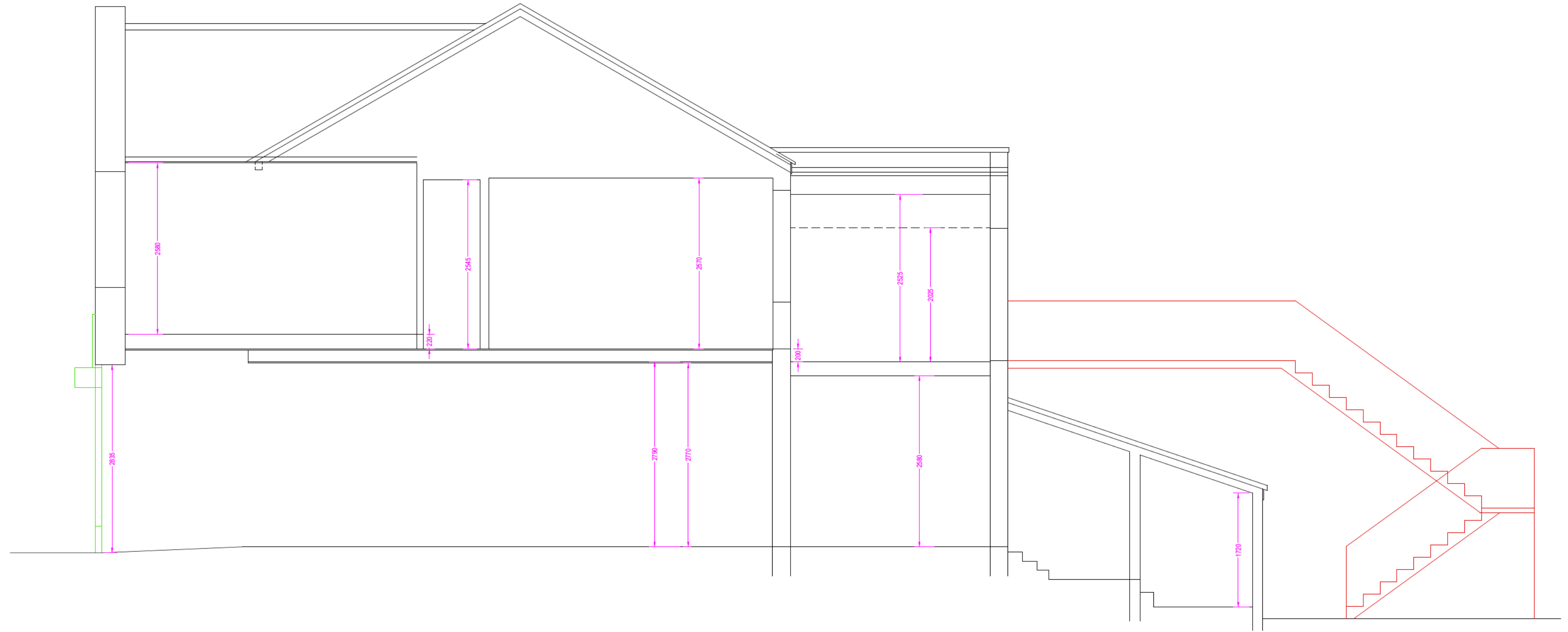
EXISTING SECTION 1:50 @ A2
