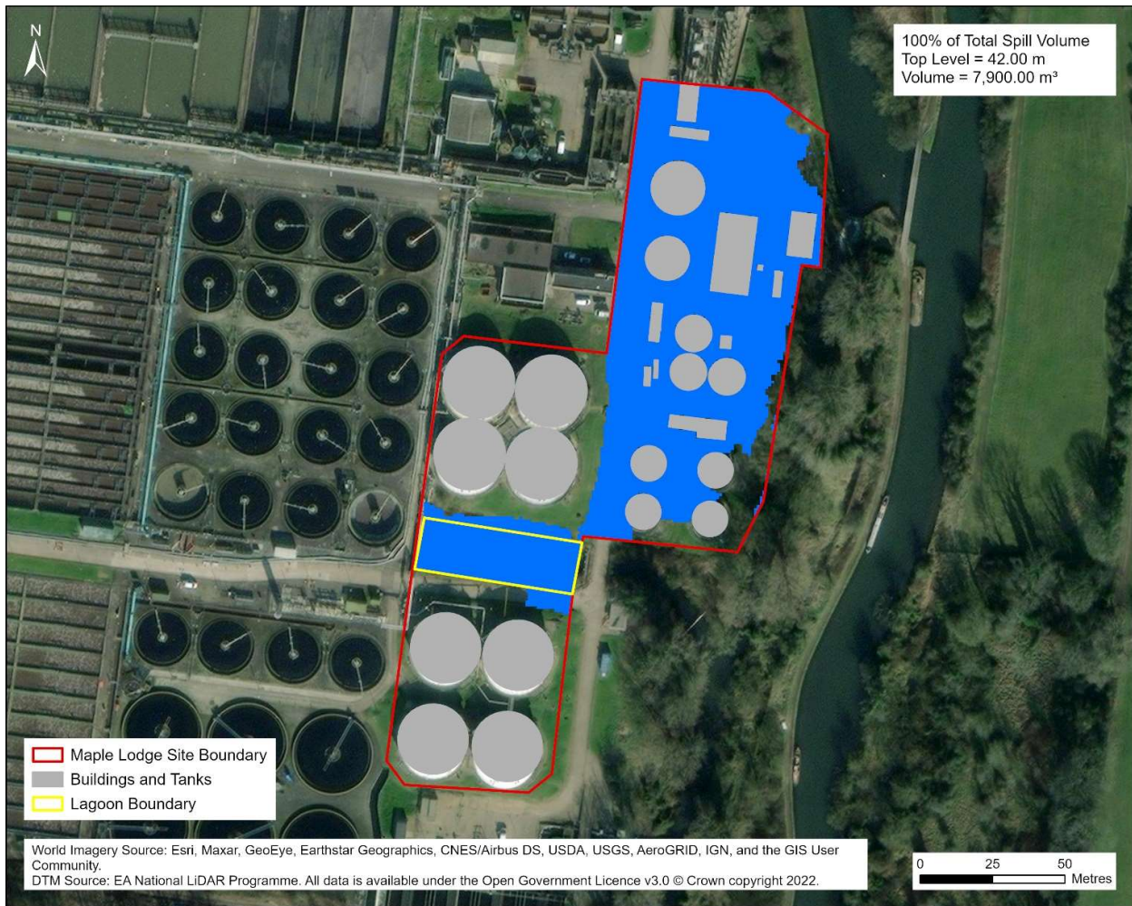
Figure 3-5 – Northern Primary Digesters and SAS asset area contained model
