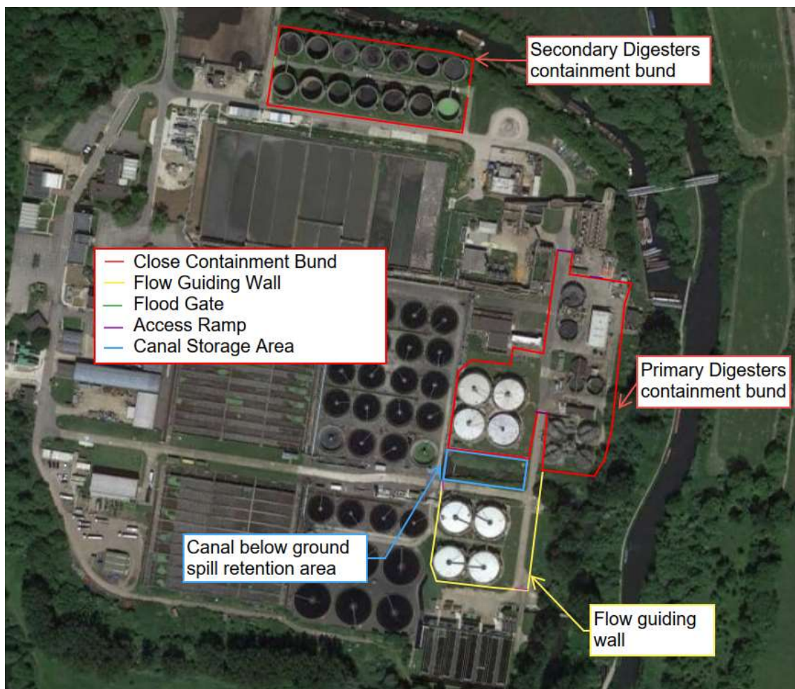
Figure 1-1- General Layout of Proposed Solution
