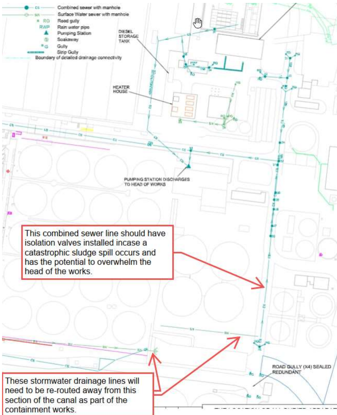
Figure 5.2 – Site Drainage Plan
