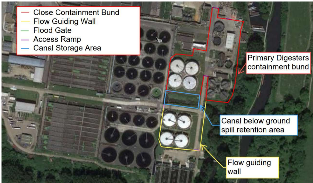
Figure 4-3 – Focus on the Primary Digesters Containment Area
