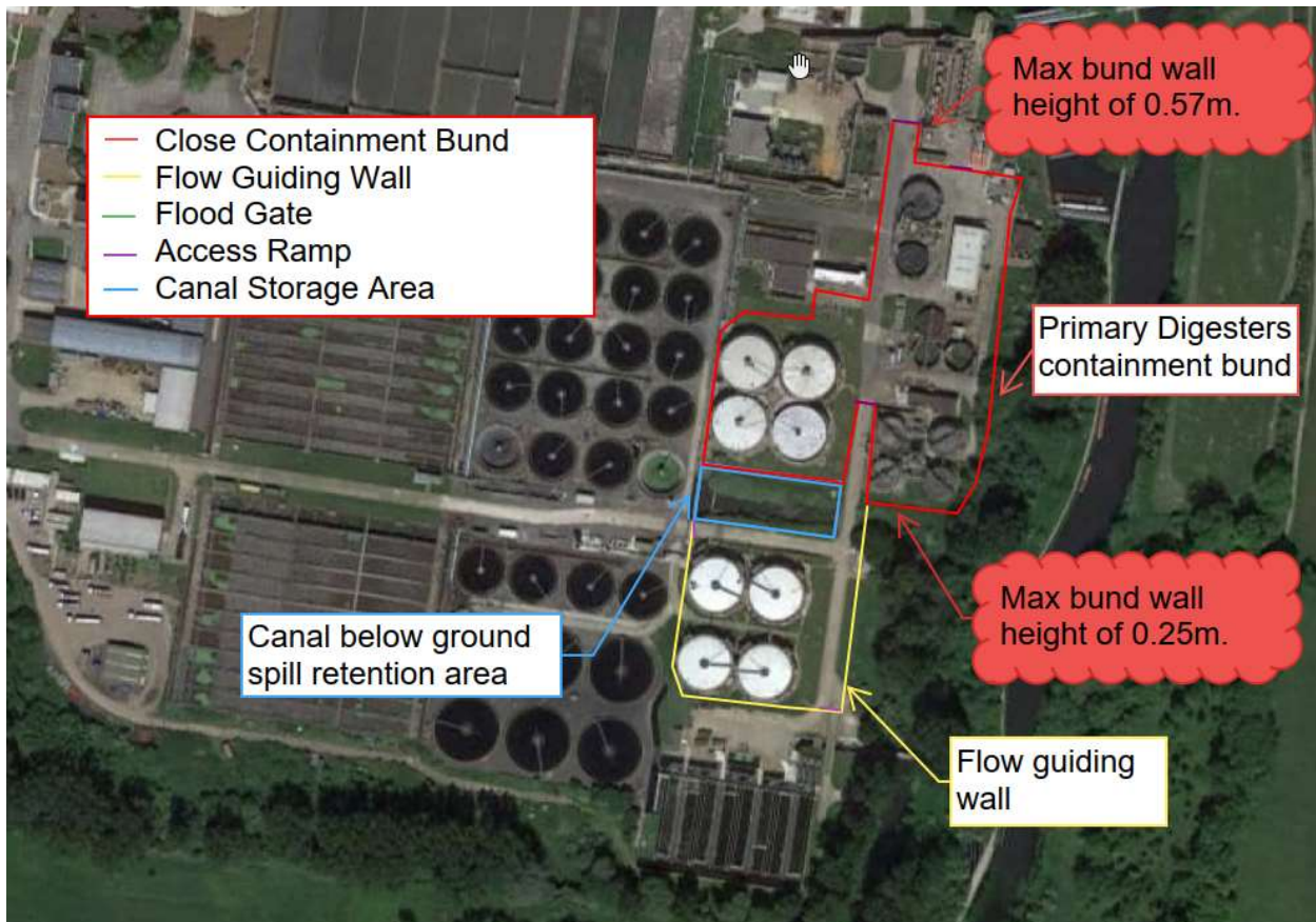
Figure 3-4 – Primary Digesters Area Containment Bund Wall Height
