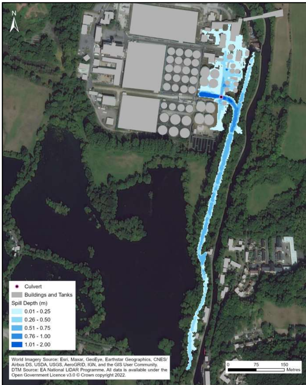
Figure 3-2 - Map of Uncontained spill event at Maple Lodge STW
