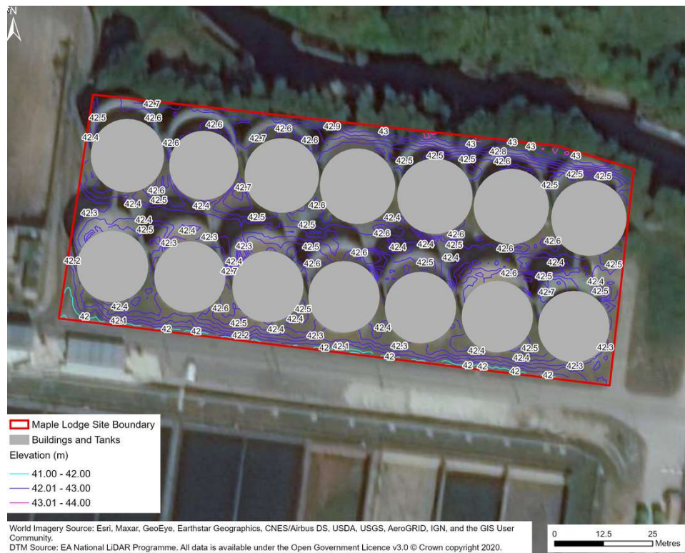
Figure 3-9 - Contour Plot of Secondary Digesters Area
