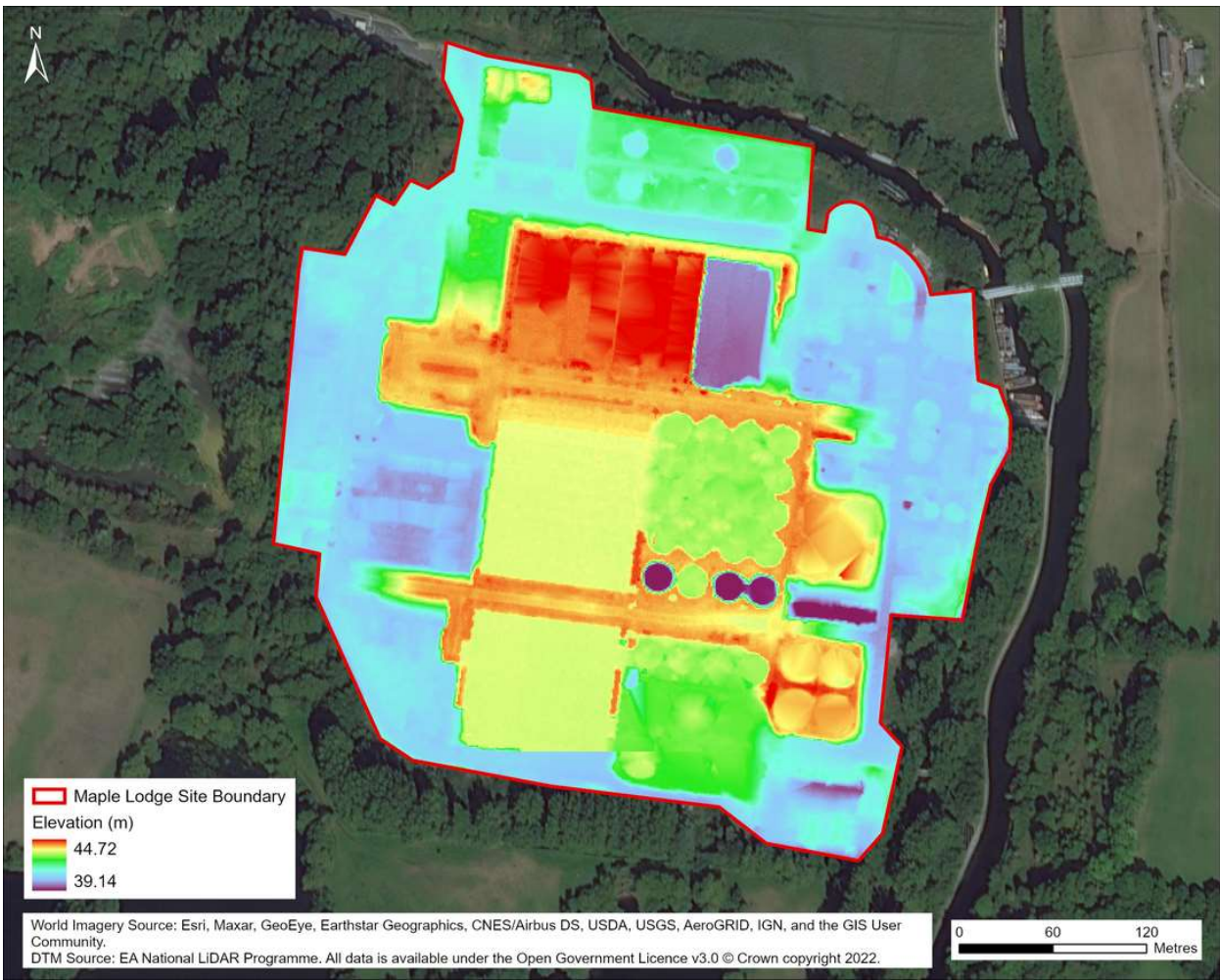
Figure 3-7 - Digital Terrain Model of Maple Lodge Sewage Treatment Works
