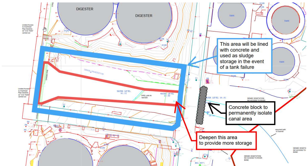
Figure 4-2 - Option 1 Canal Storage Area
