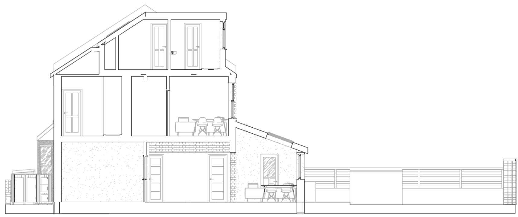
SECTION AA
