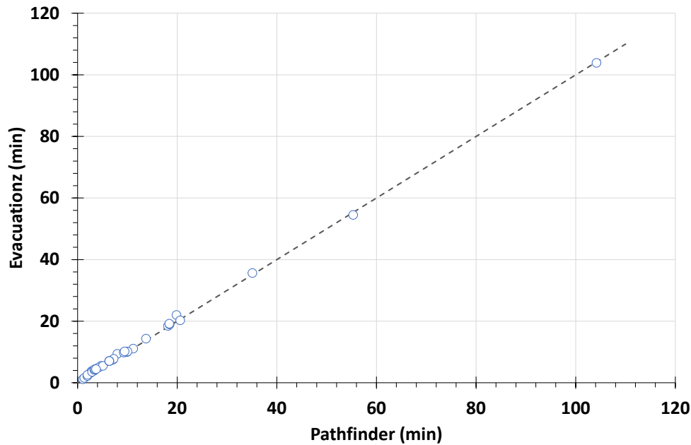
Figure A3-28 Comparison between evacuation times produced by Pathfinder and Evacuatzionz for Scenarios B1–B30
