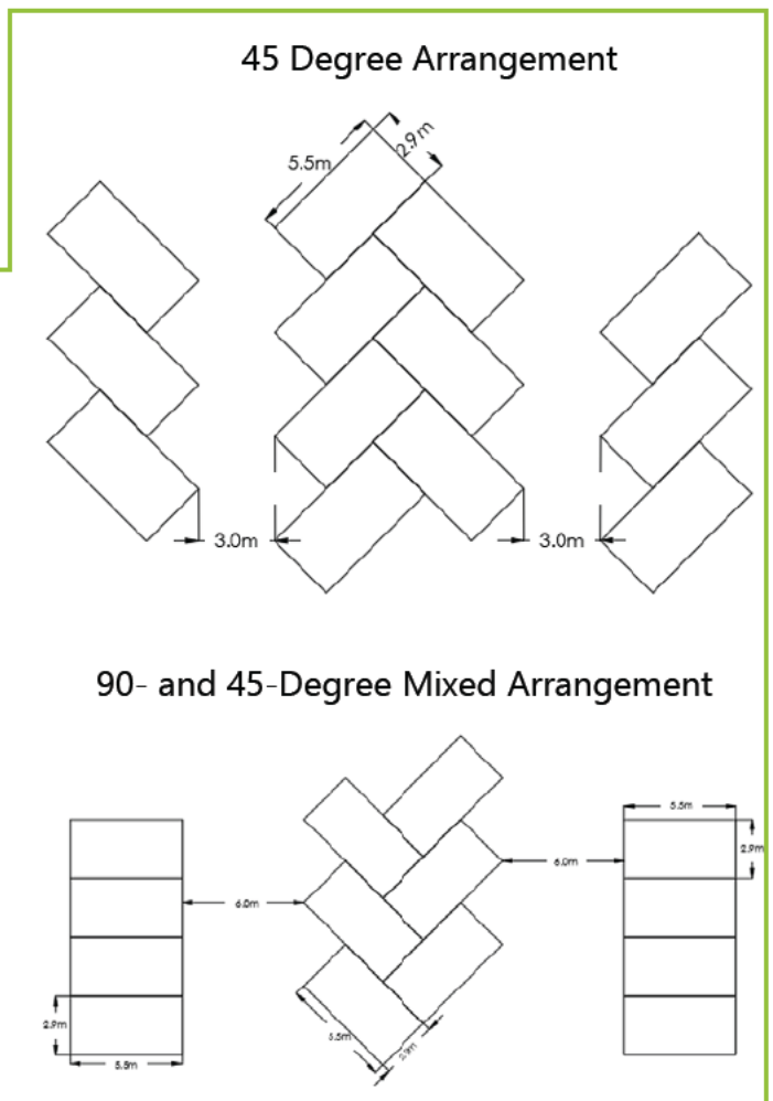
Figure 7-6: Mixed, 45 Degree and 90 Degree Arrangements
