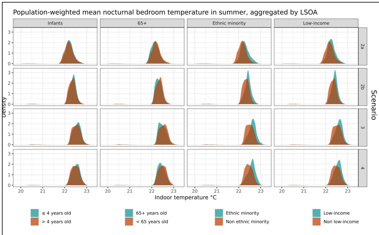
Figure 17. The population-weighted mean nocturnal bedroom temperature in summer for different population groups, across the four building intervention scenarios for English LSOAs, in 2030s time horizon under RCP 2.6.
