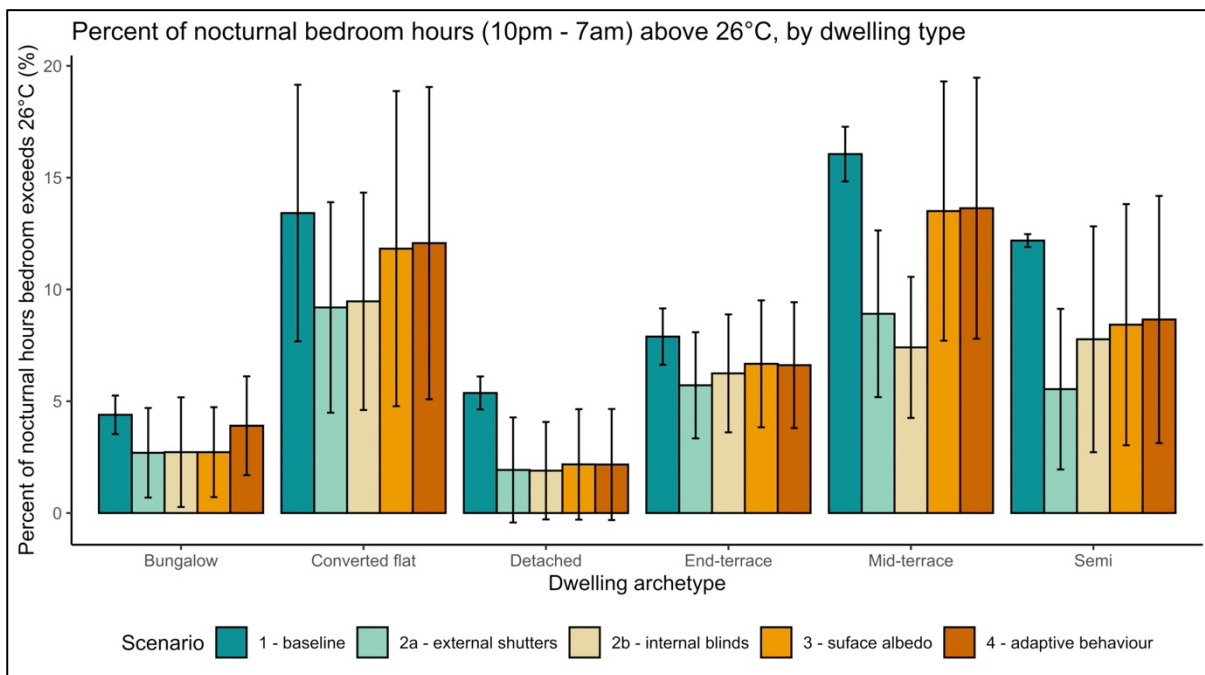
Figure 47. The percent of annual night time hours the bedroom temperature exceeded 26C in the 2050 time horizon under 1.5C warming, by dwelling type, across all building intervention scenarios for the Scottish housing stock.
