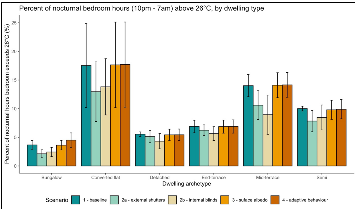
Figure 30. The percent of annual night time hours the bedroom temperature exceeded 26C, by dwelling type, across all scenarios for Northern Irish stock, at 2030s time horizon under RCP 2.6.
