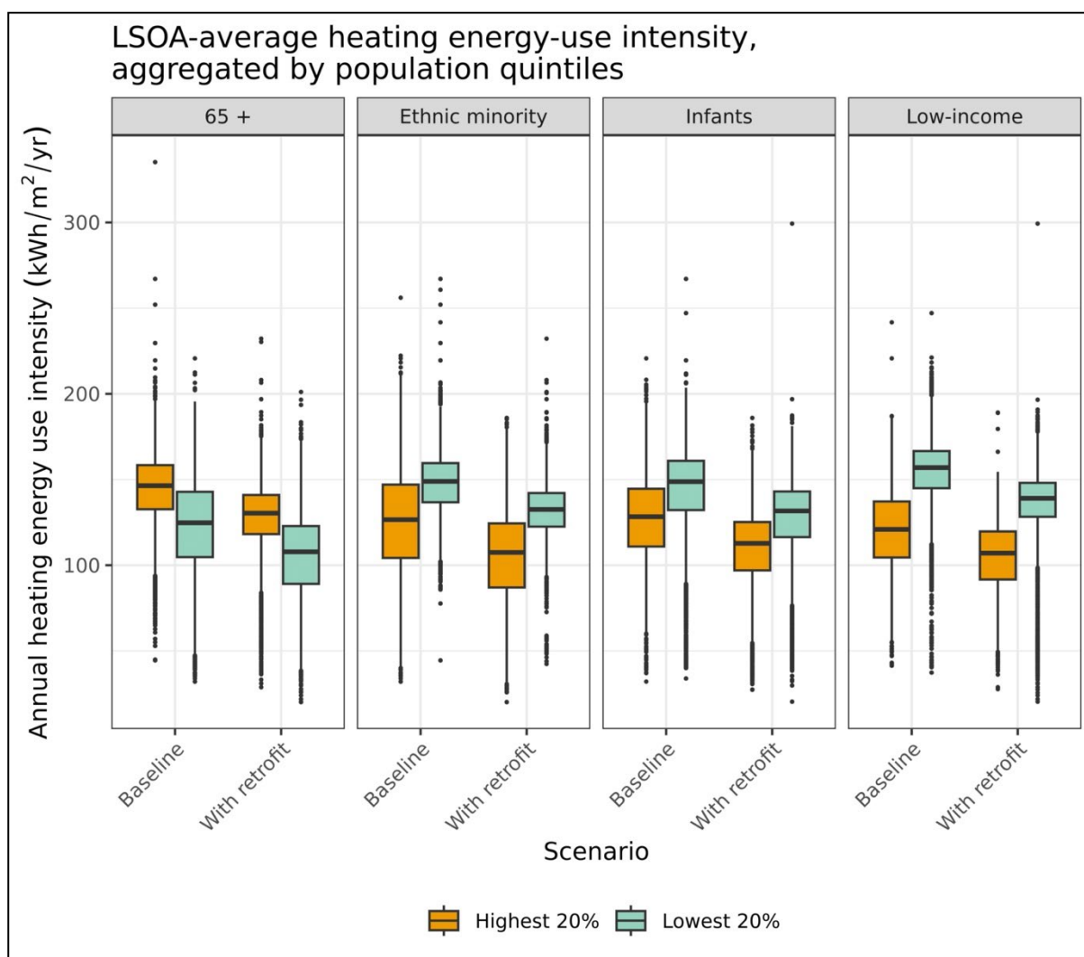
Figure 8. LSOA-average heating energy-use intensities (EUI) for each population subgroup under baseline English housing stock conditions and with retrofit measures under the 2030 RCP emission scenario.
