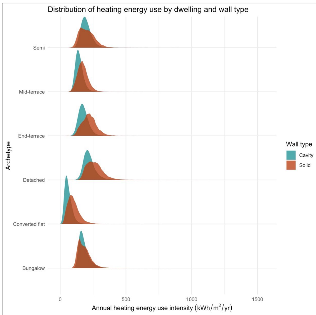
Figure 25. The distribution of heating energy use intensities ( \text{kWh/m}^2/\text{yr} ) by dwelling and wall type for the baseline Northern Irish housing stock, in the 2030s time horizon under RCP 2.6.
