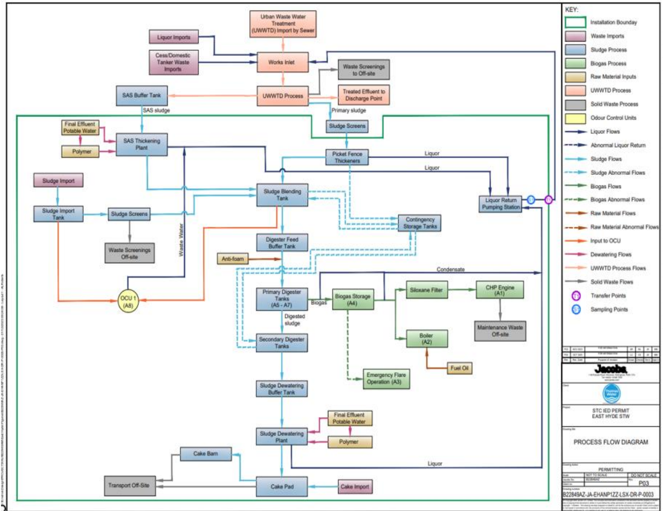
Source: STC IED Permit East Hyde process flow P03.
