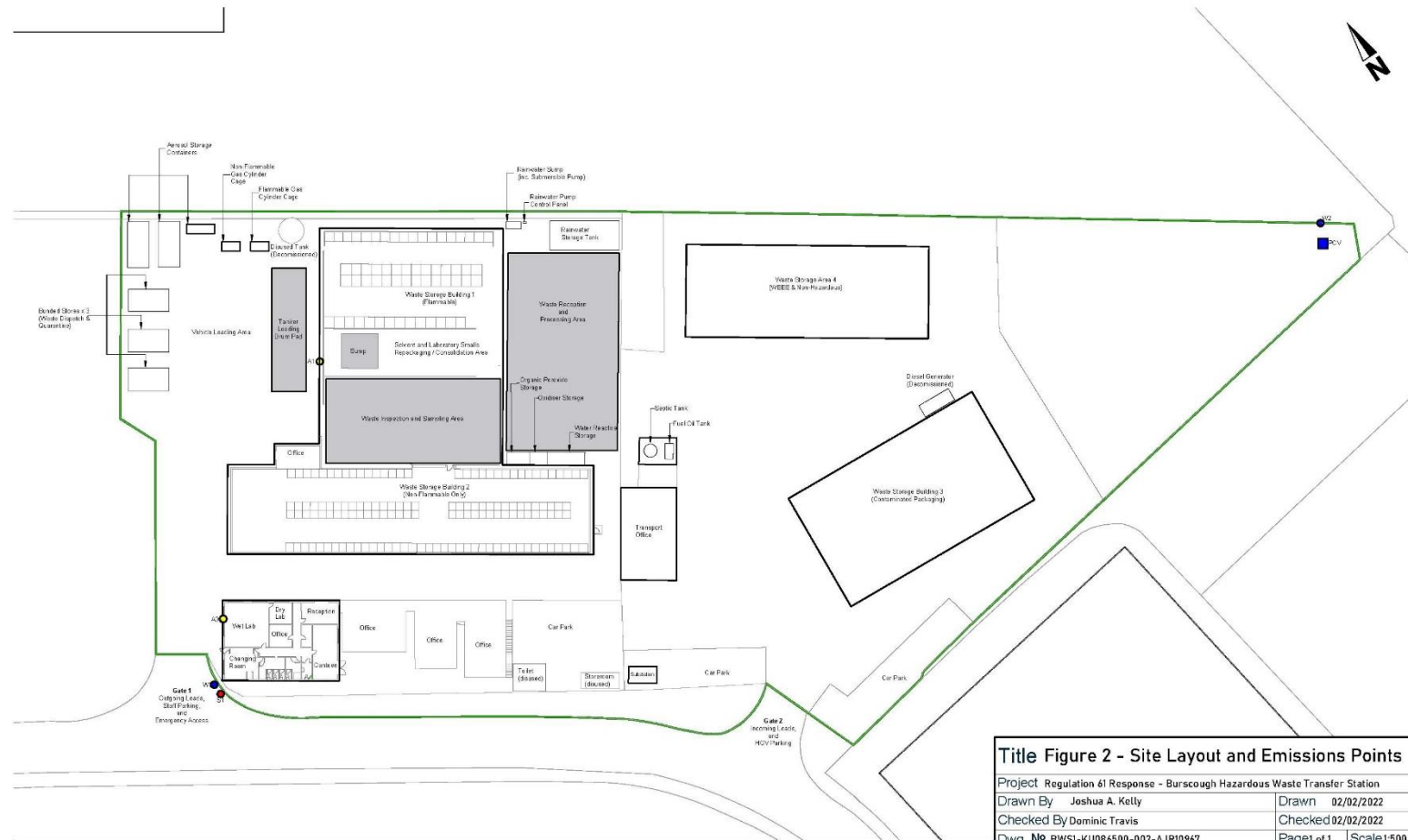
Figure 2: Site Layout Plan including emission points
