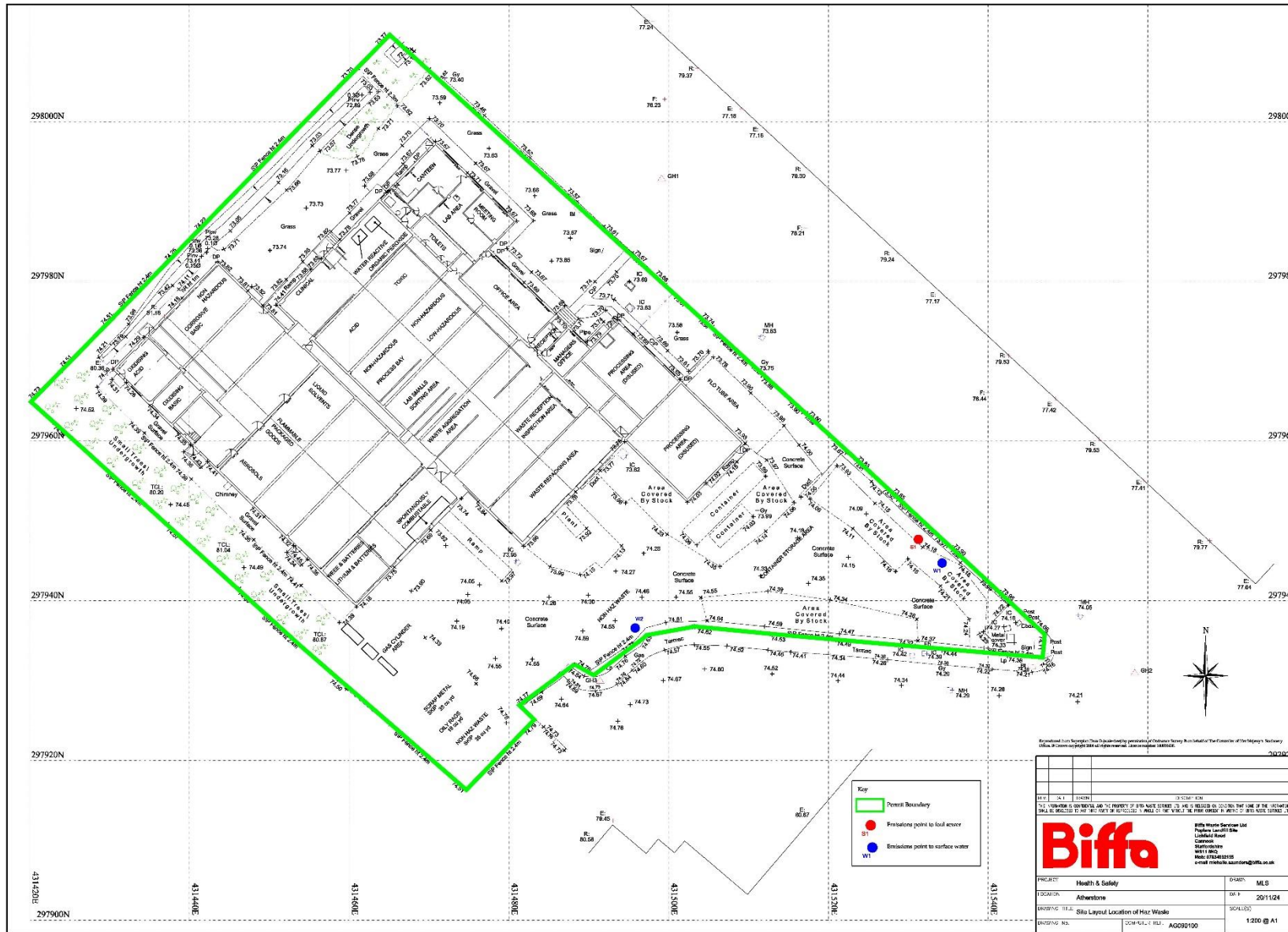
Figure 2: Site layout plan and permit boundary.
