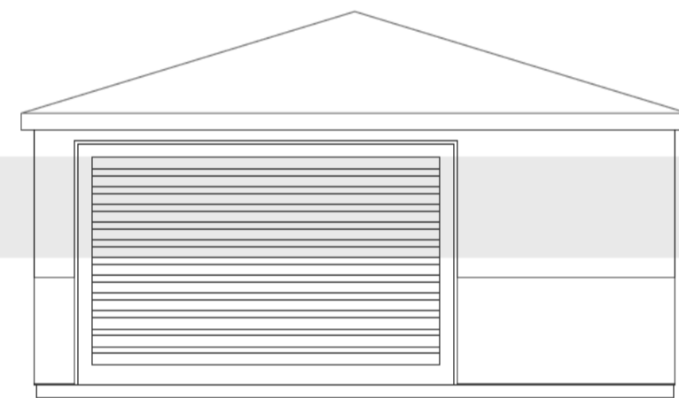
11 Proposed Garage Front Elevation Scale: 1:50
