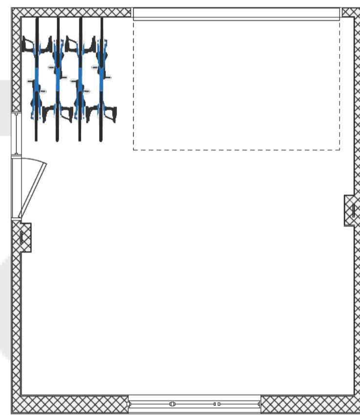
8 Proposed Garage Floor Plan Scale: 1:50
