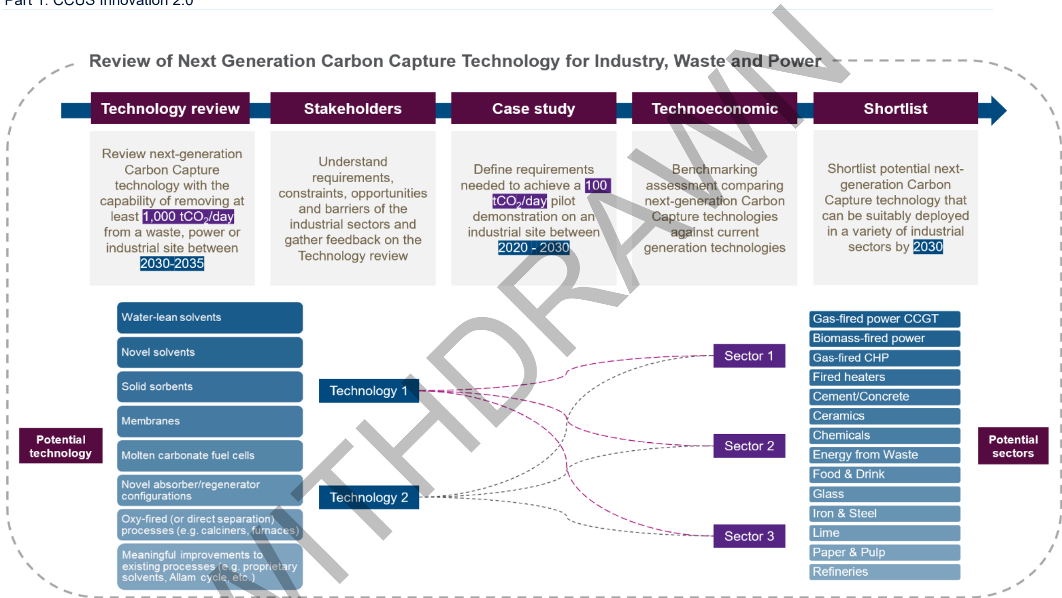
Figure 5: Methodology used in the review of Next Generation Carbon Capture Technology
