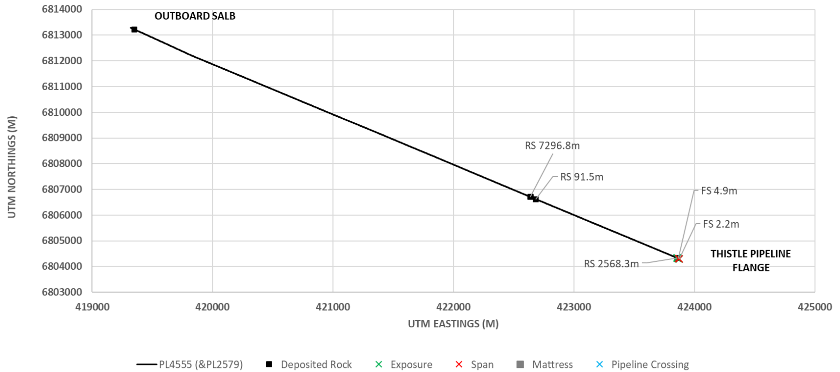
Figure 6.3.3 PL4555 (PL2579) pipeline route (2019)
