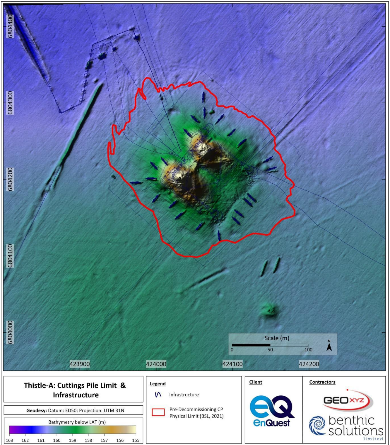
Figure 4.3.1 Thistle Cuttings Pile Physical Boundary [31]
