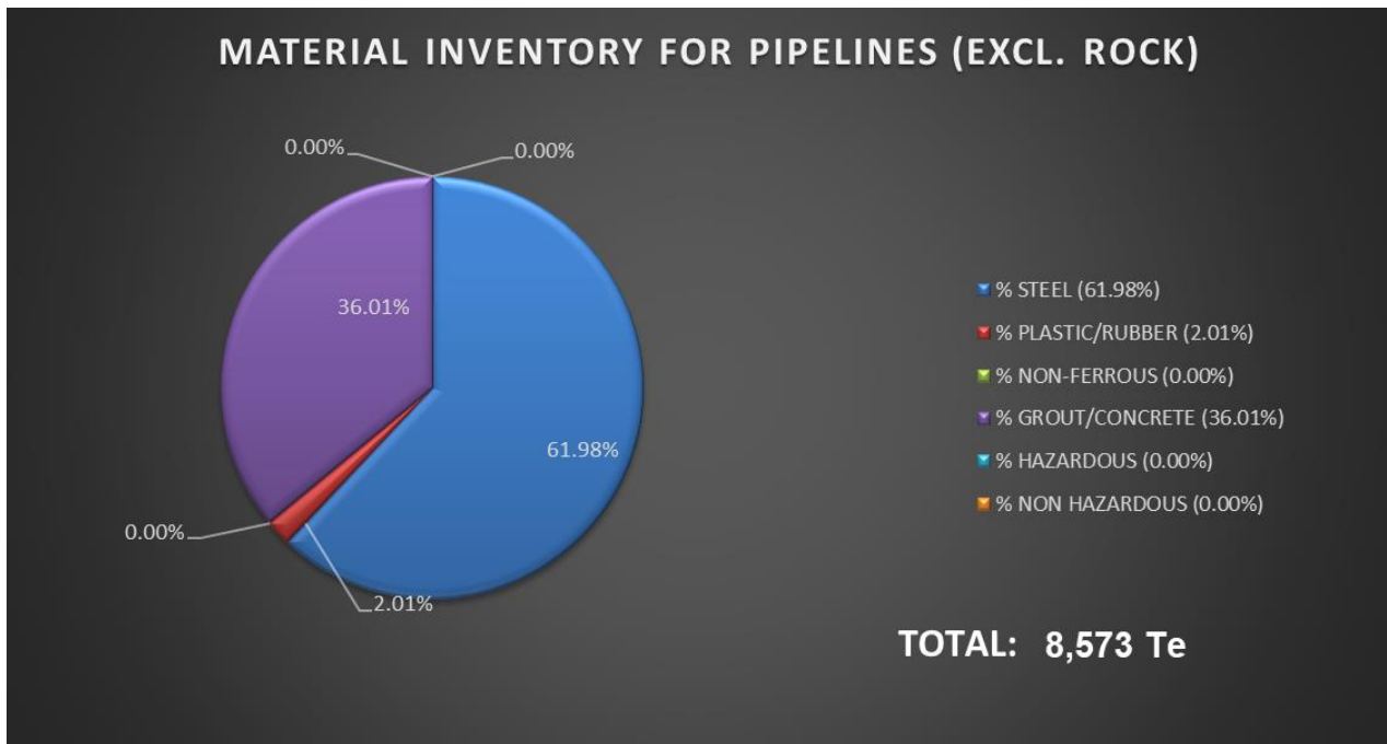
Figure 3.10.3 Estimated material inventory for Thistle pipeline(s) 1
