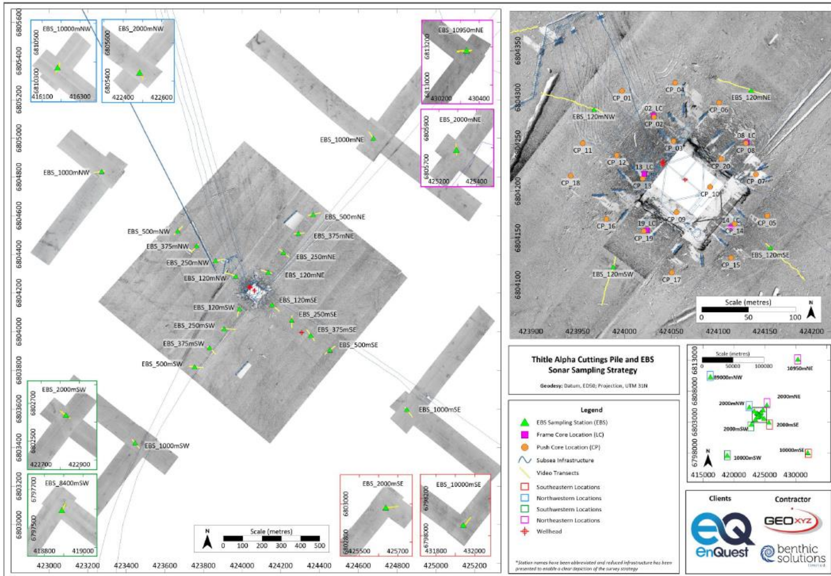
Figure 4.1.1 EBS and cuttings pile sample stations around Thistle platform [30][31]
