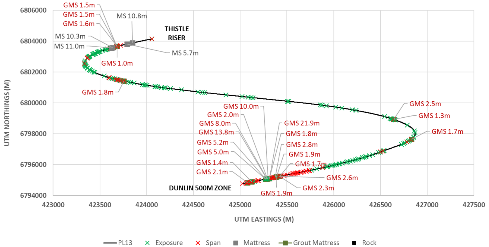
PL13 16in Thistle to SPM pipeline routing plot UTM coordinates (2018)
