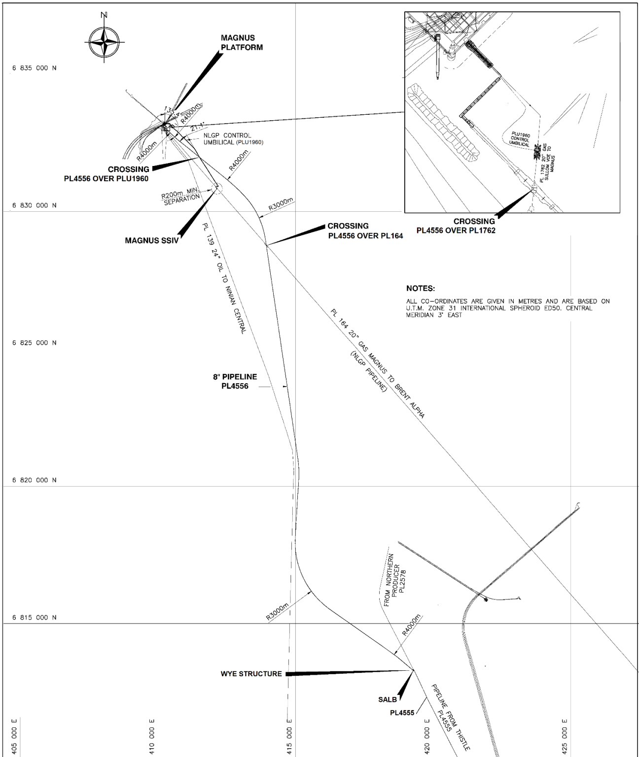
Figure 3.5.1 PL4556 pipeline crossings
