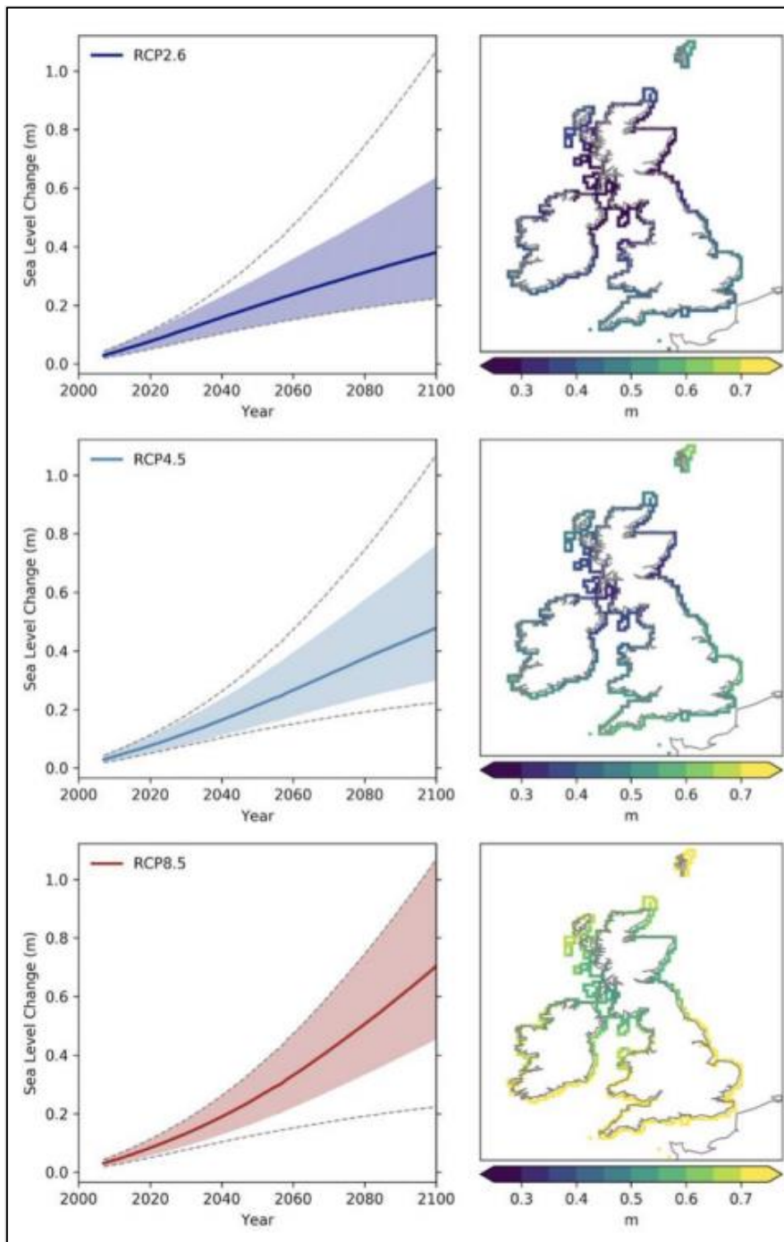
Figure 3. Model outputs showing UK average sea level projections under different emissions scenarios up to the year 2100 ( left ); and spatial visualisation of the projected sea level change across the UK at 2100 for the three emissions scenarios ( right ) (Taken from MCCIP, originally from the UKCP18 Marine Report)
