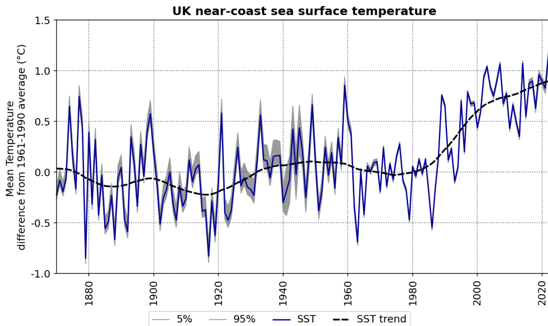
Figure 4: UK annual mean sea surface temperature (SST) in near-coastal waters from 1870-2023, (expressed as anomalies relative to the 1961-1990 long-term average) (Taken from the 'State of the UK Climate 2023' report (Kendon et al., 2024))
