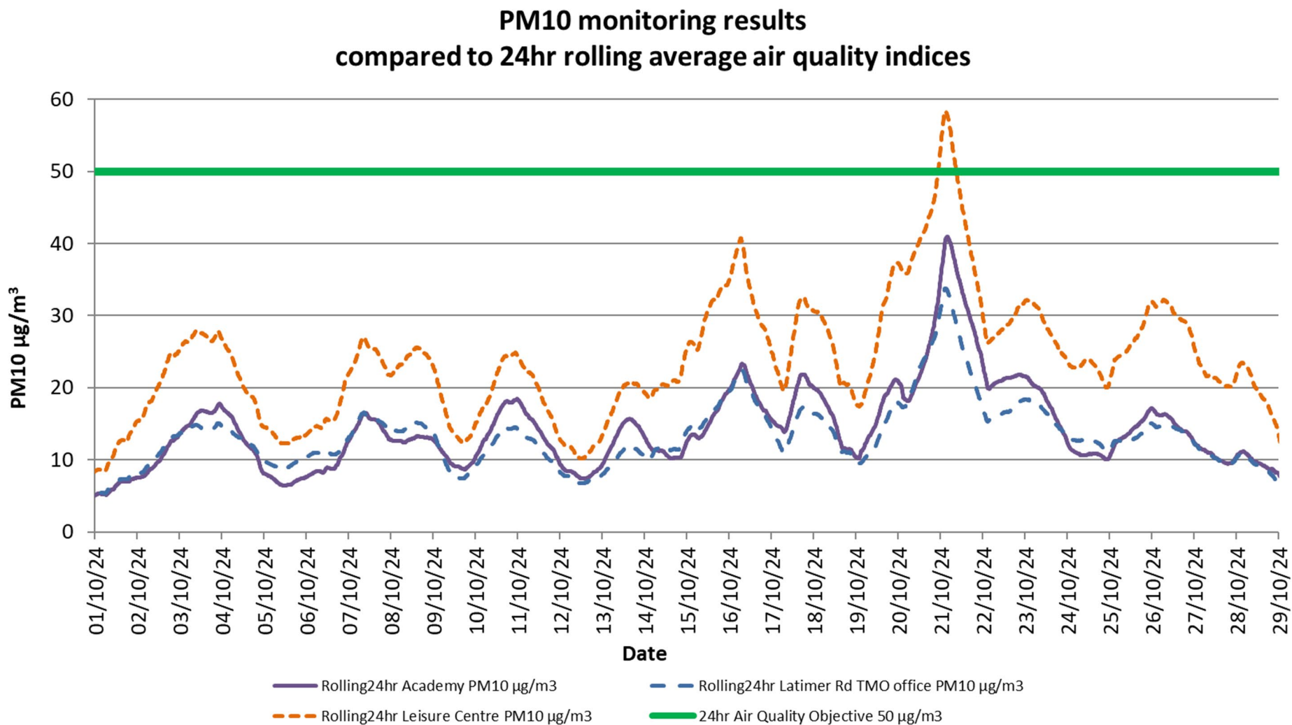
Figure 3. 24-hour average particulate matter (PM 10 ) concentrations over the last 4 weeks for each of the 3 UKHSA commissioned monitoring locations: Kensington Aldridge Academy, Kensington Leisure Centre and Latimer Road TMO office location
