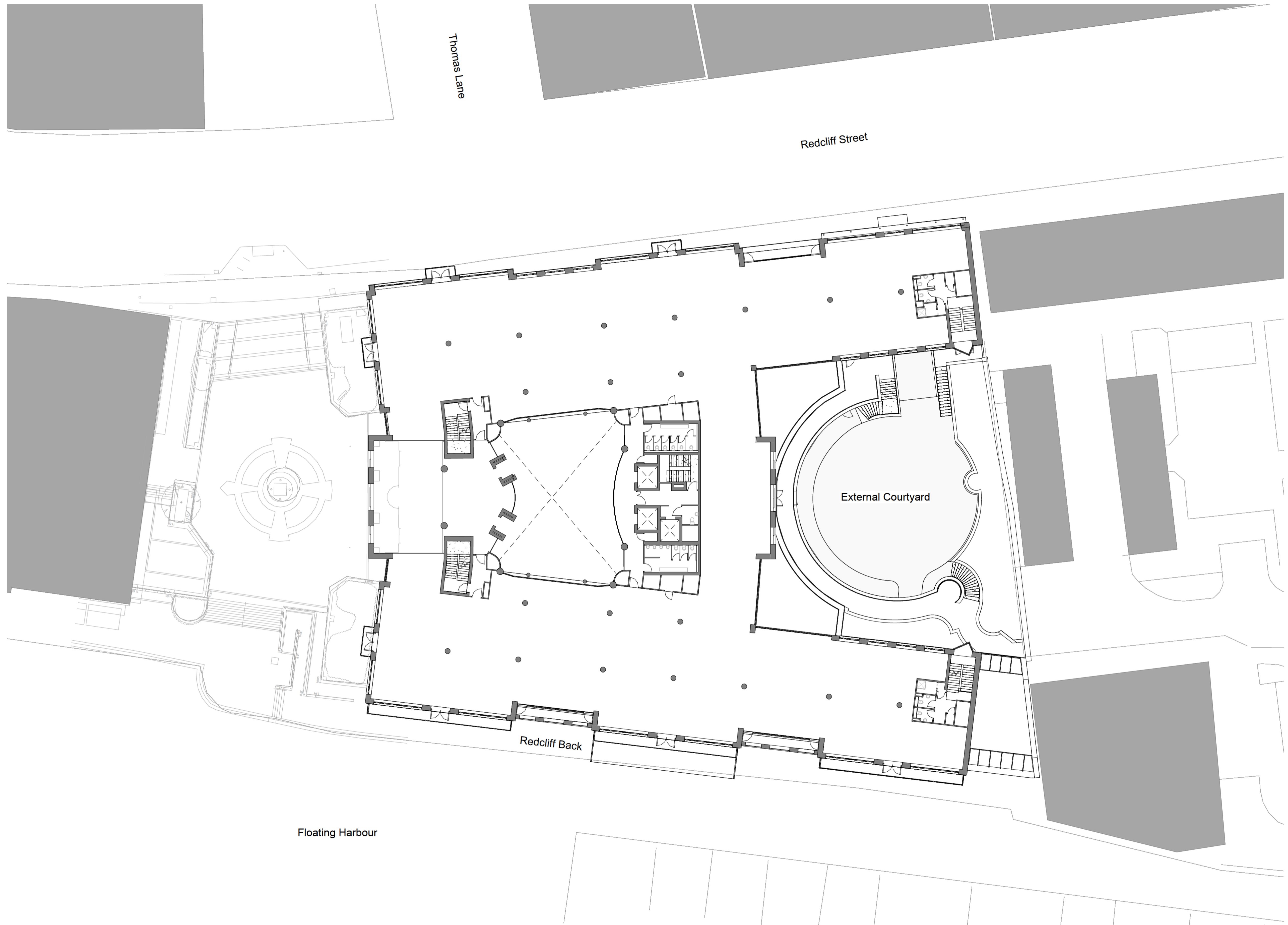
Existing Building - Third Floor Plan - Planning 1 : 200
