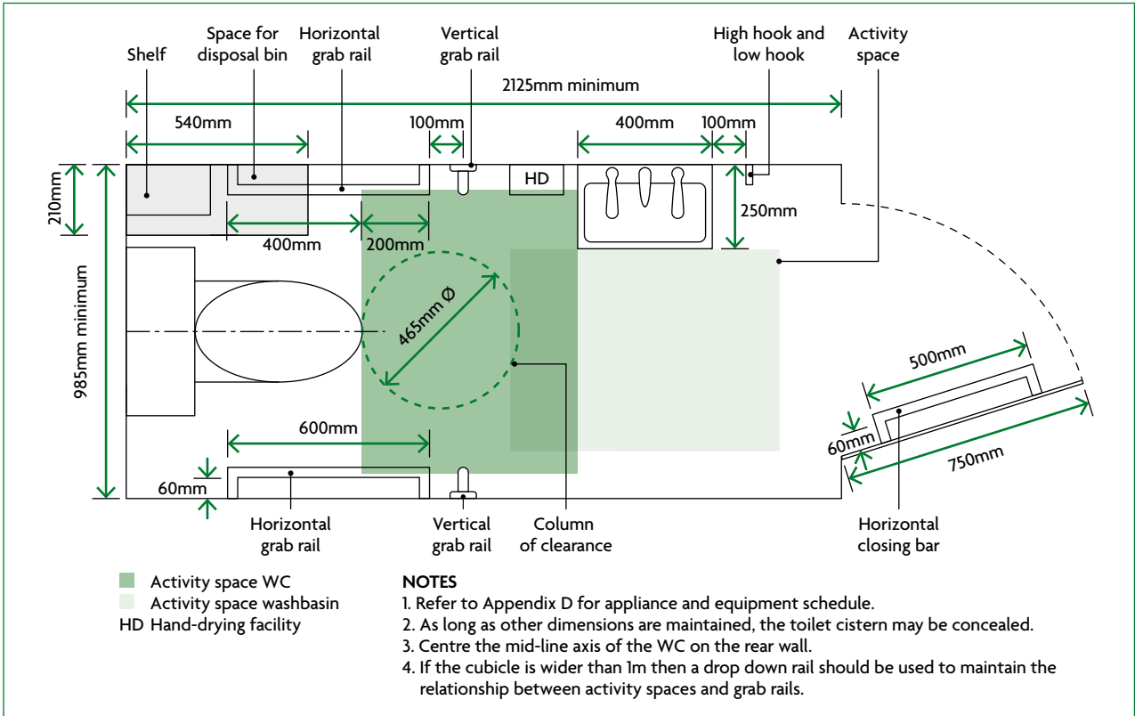
Diagram 3.1 Type A, plan view showing minimum dimensions
