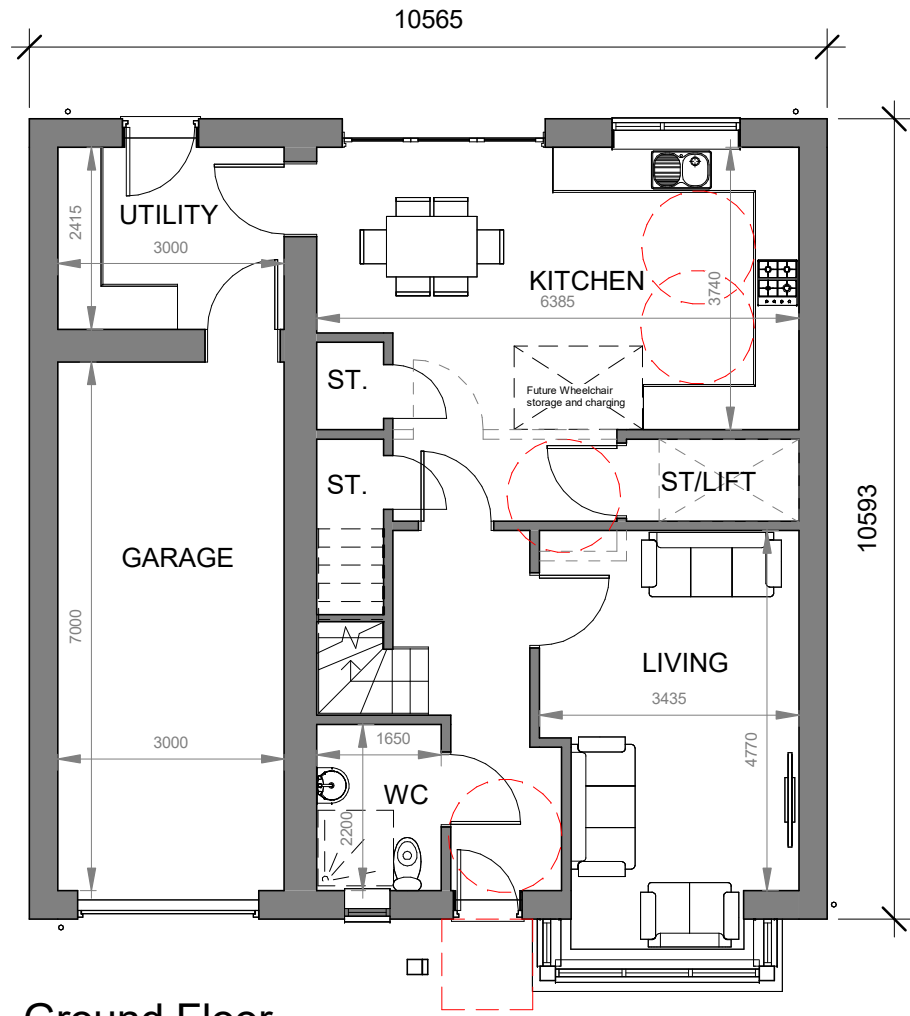
Ground Floor 1 : 100
