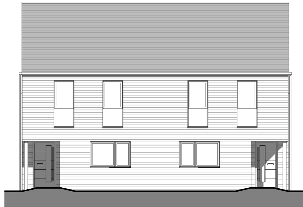
Front Elevation 1 : 100
