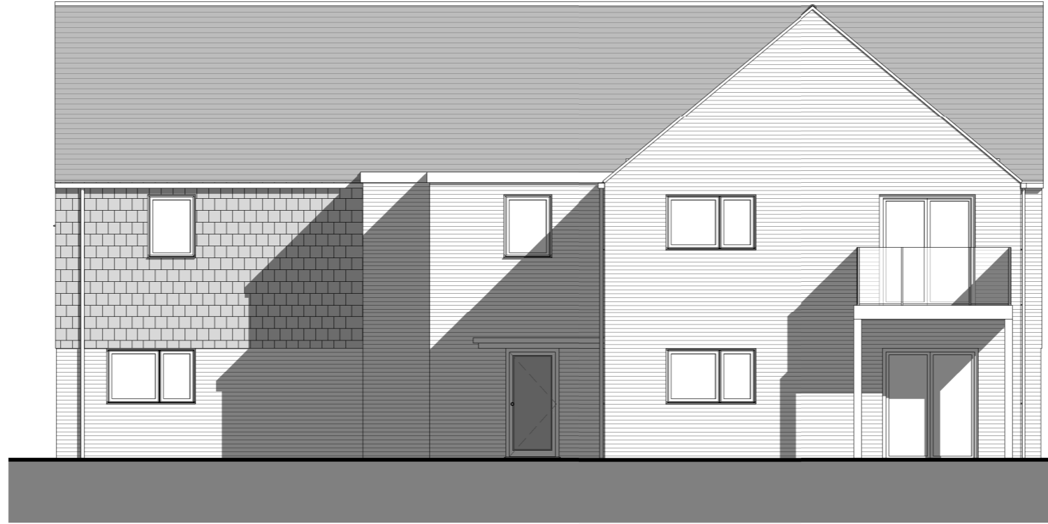
REAR ELEVATION
