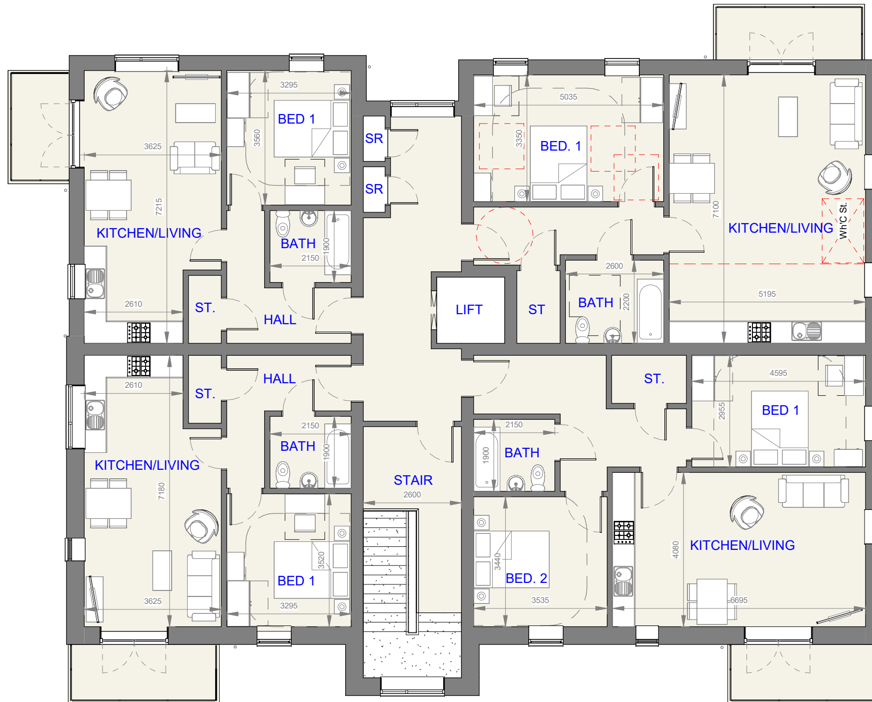
FIRST FLOOR 1 : 100
