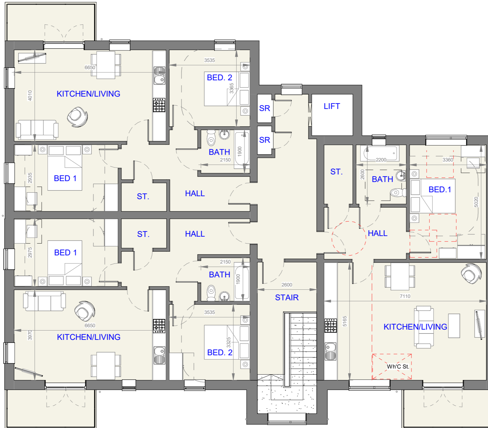
FIRST FLOOR 1 : 100
