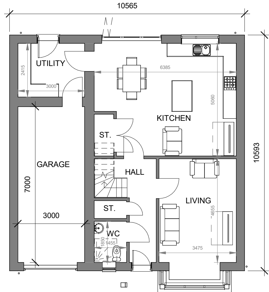
Ground Floor 1 : 100
