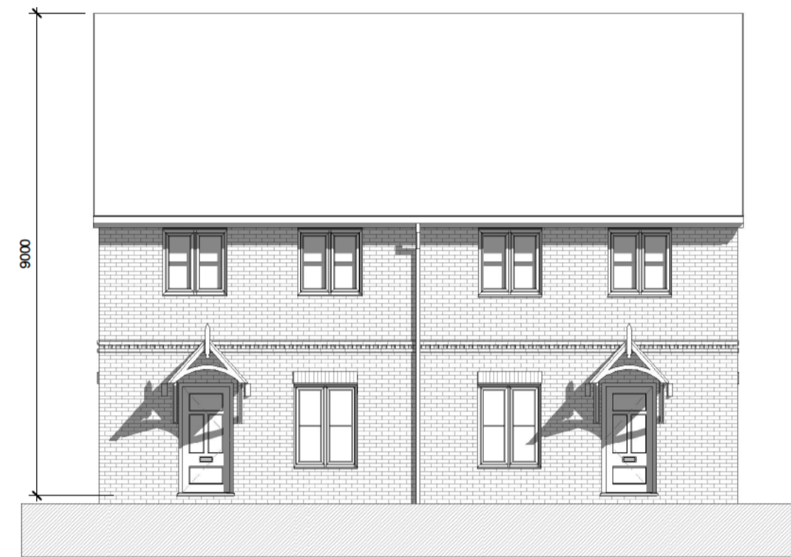
Front elevation 1 : 100
