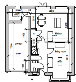
Ground floor 1:100
