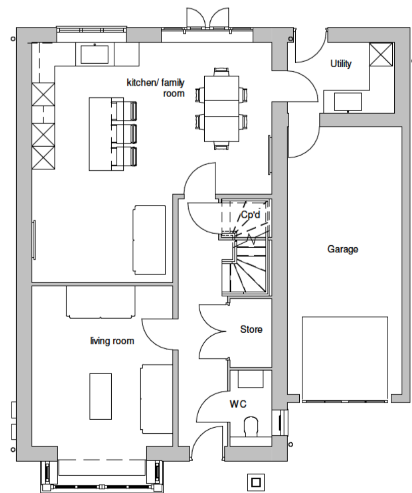
Ground floor 1 : 100
