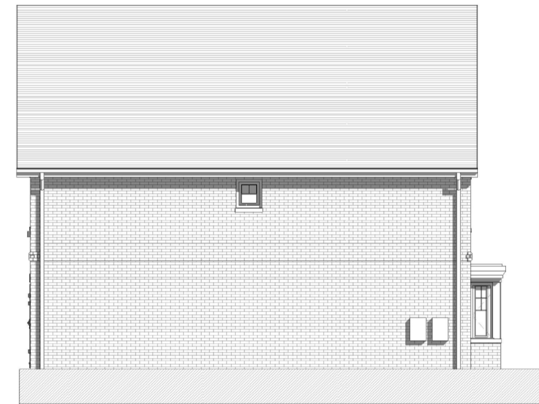
Side (left) elevation 1 : 100
