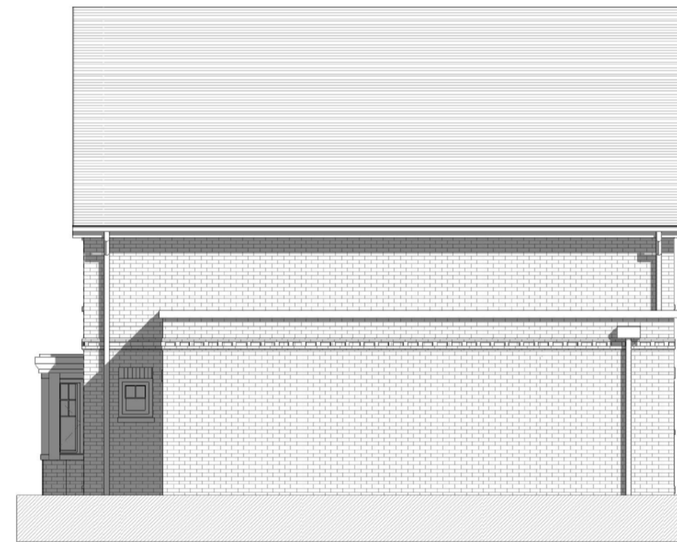
Side (right) elevation 1 : 100
