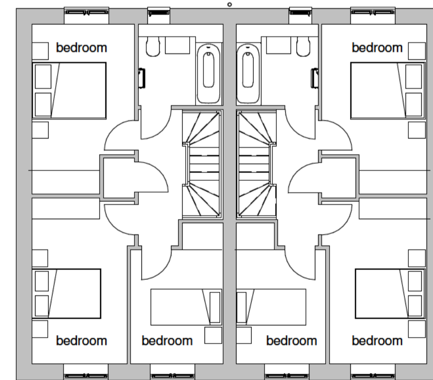
First floor 1 : 100
