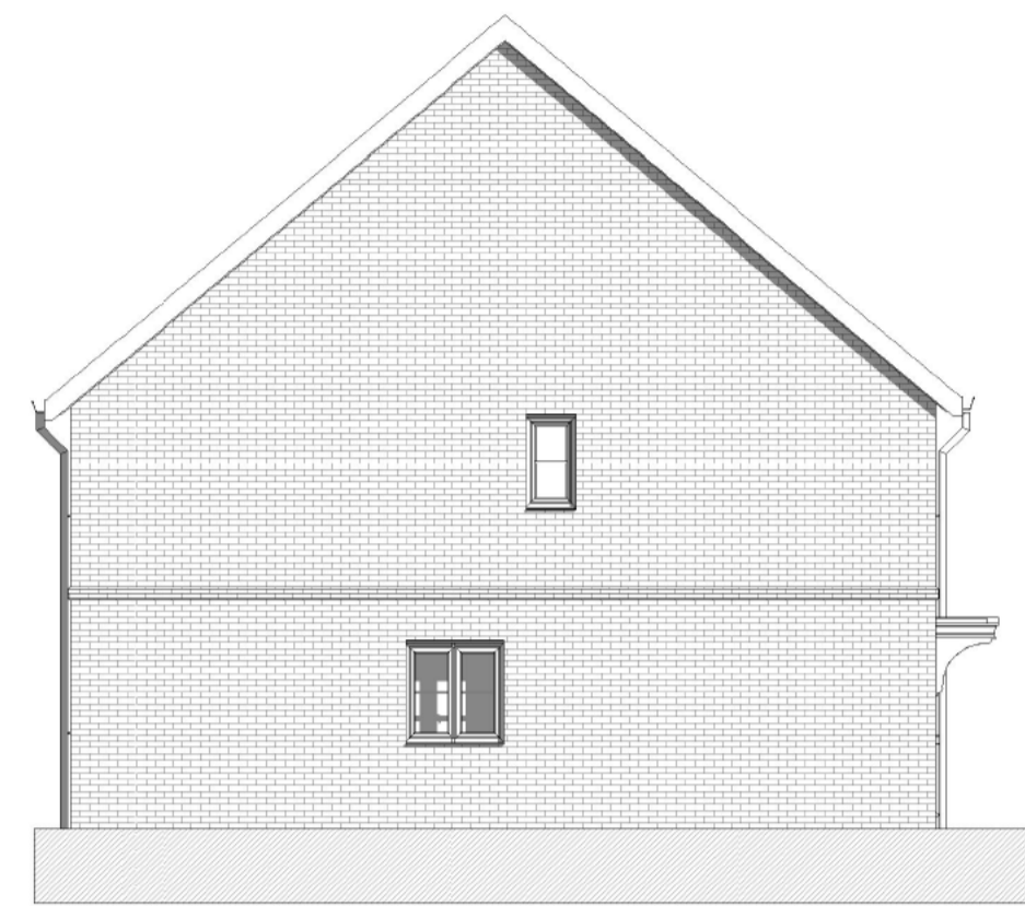
Left elevation 1 : 100
