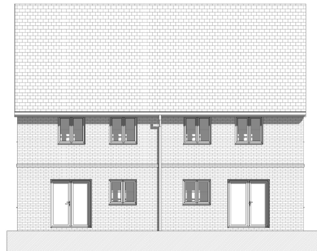
Rear elevation 1 : 100
