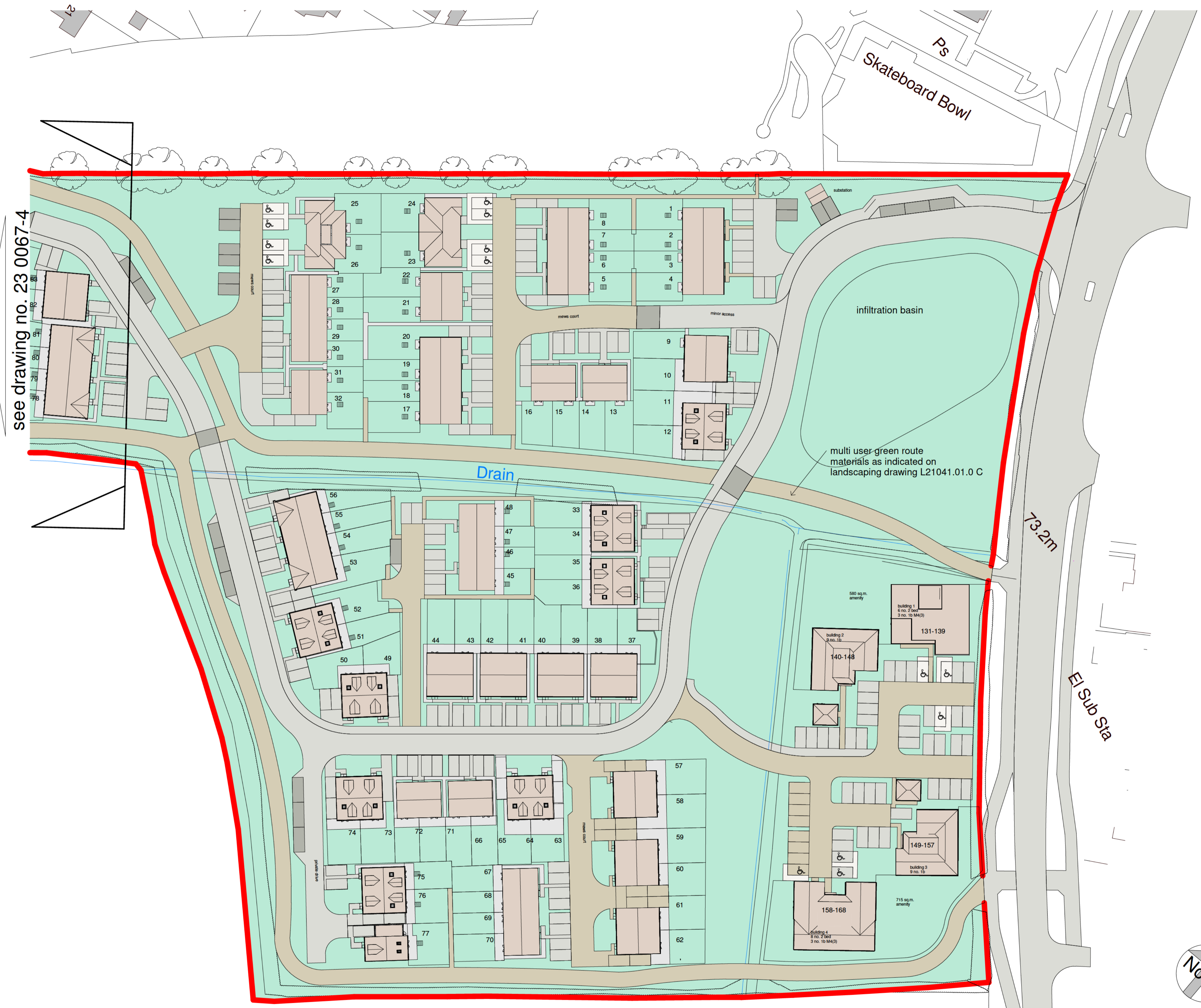
Block plan-North 1 : 500
