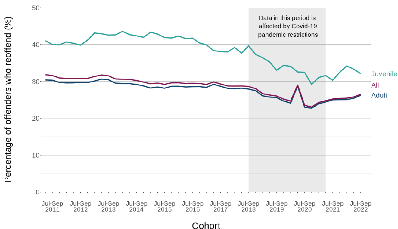
Figure 2: Percentage of adult and juvenile offenders 1 in England and Wales who commit a proven reoffence, by quarter, April to June 2011 - July to September 2022 (Source: Table A1)
