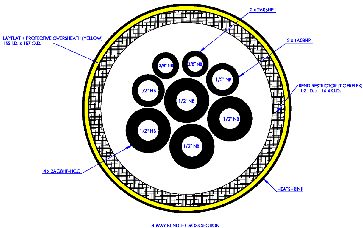
Figure A.5.1: Well P3 hydraulic fly-lead PLU4976 construction
