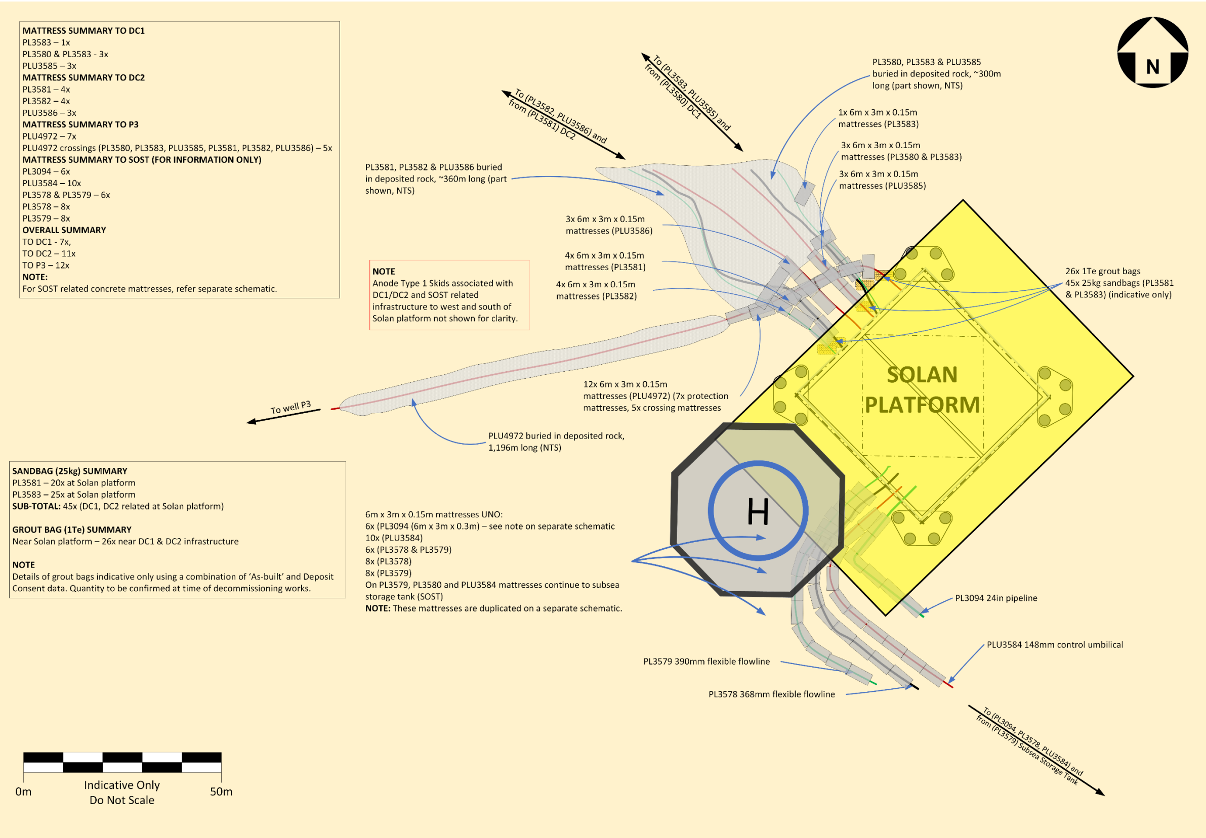
Figure B.21: Pipelines, flowlines & umbilicals at the Solon platform
