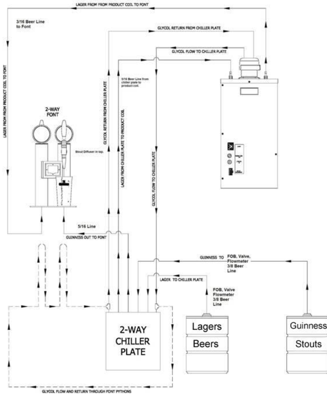
Figure 2 - Flow schematic
