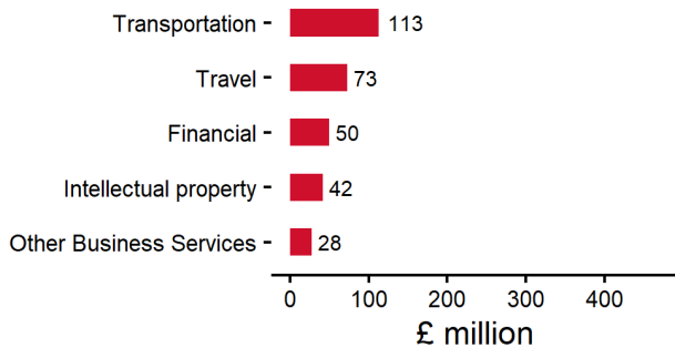
The top 5 UK services exports, in the four quarters to the end of Q4 2023, to Iceland
