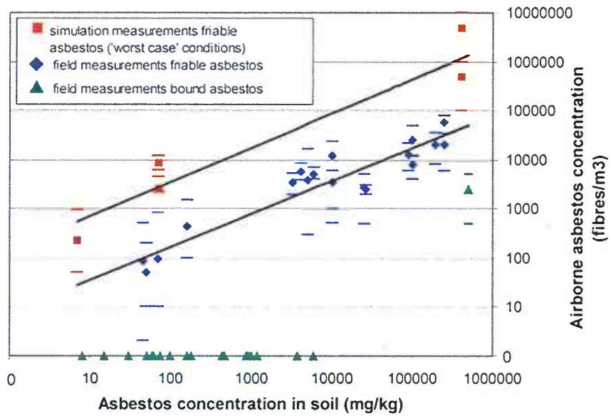
Figure 2. Average airborne asbestos concentrations from several comparable measurements ( symbols ) in \text{fibres/m}^3_{\text{air}} and 95% confidence intervals ( hyphens ), from worst case simulation experiments ( squares ) and from field measurements with friable ( diamonds ) and bound ( triangles ) asbestos, as a function of asbestos concentration in soil. Straight lines represents the 95% confidence intervals of all data.
