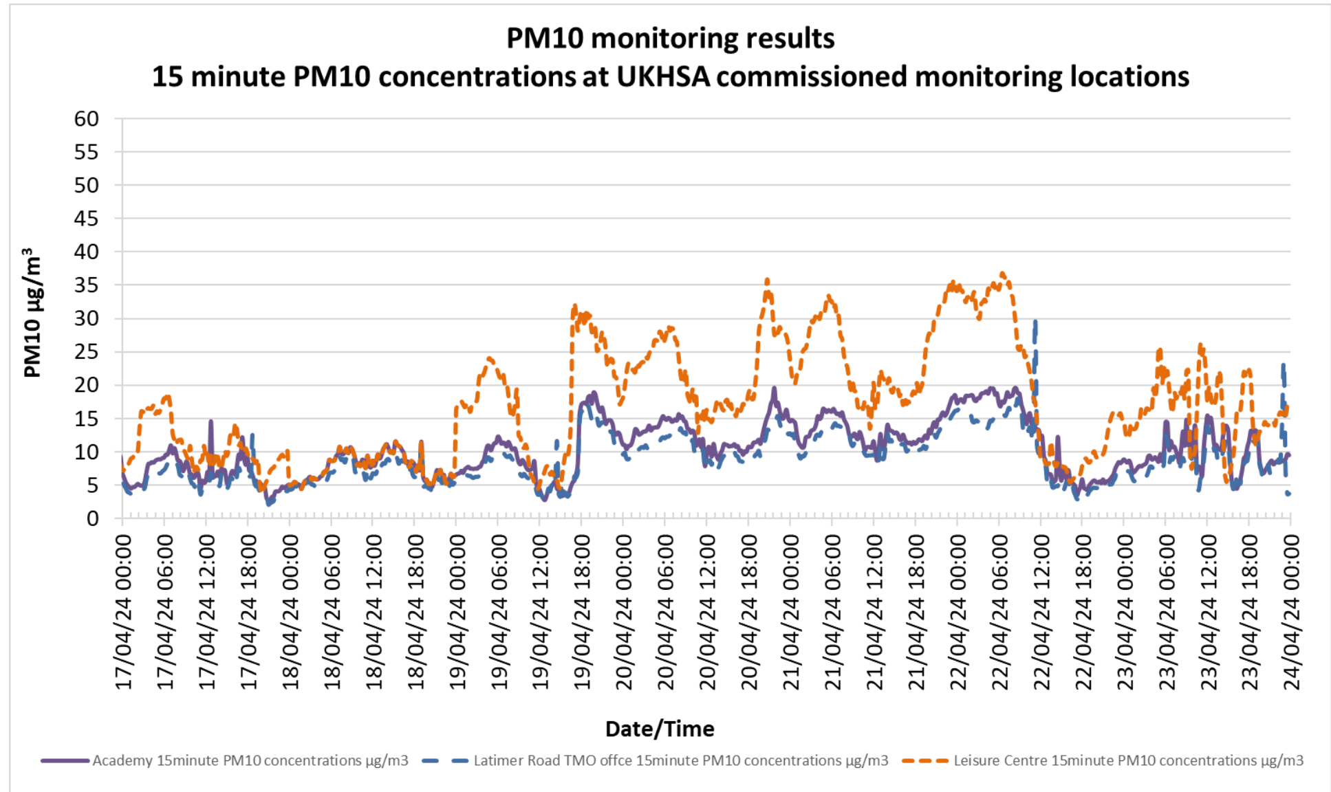
Figure 2. 15 minute particulate matter (PM 10 ) concentrations over the last week for each of the 3 UKHSA commissioned monitoring locations: Kensington Aldridge Academy, Kensington Leisure Centre and Latimer Road TMO office location
