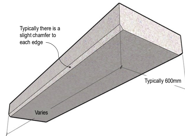
Figure 8: Typical profile of RAAC panels
