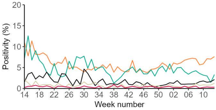
Rhinovirus
